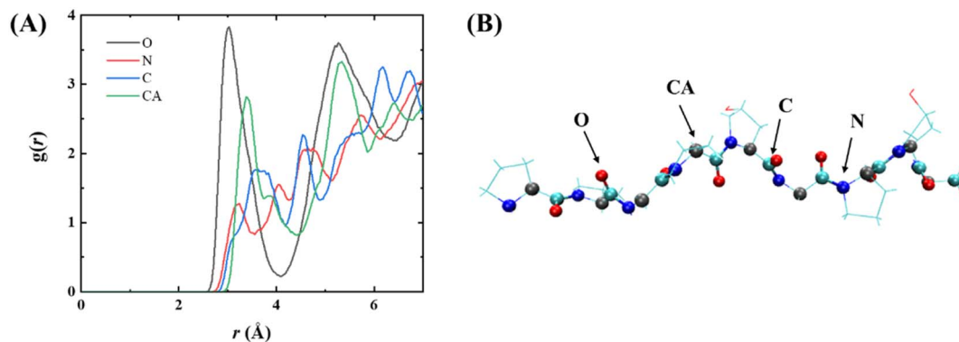
Fig. 8 (A) RDFs for the interaction of the backbone atoms of PPG-3 ( i.e. O, N, C, and CA) with gold. (B) Schematic diagram of atomic names; C atoms are aqua blue, CA atoms are grey, O atoms are red, and N atoms are blue.
