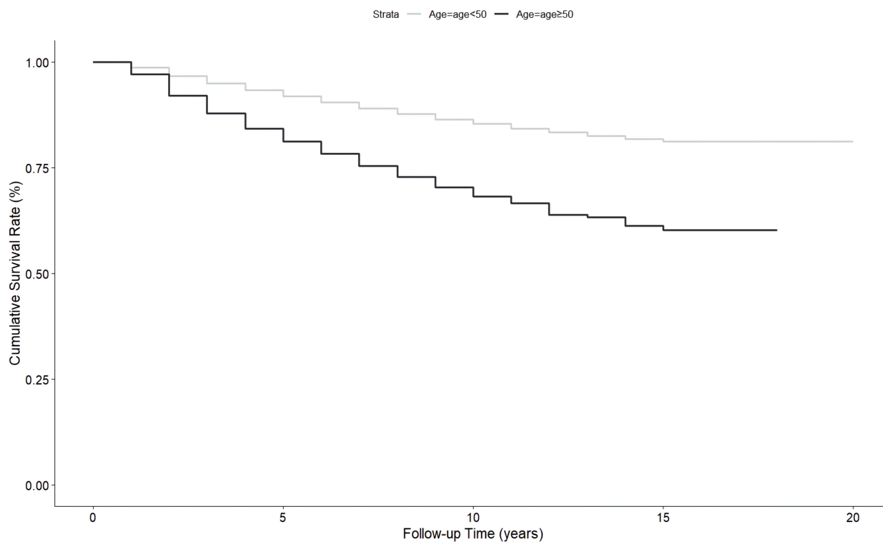
Figure 4 Cumulative survival probability of PLWH receiving ART for six months or more in different age groups in Sichuan Province, 2003–2022.
