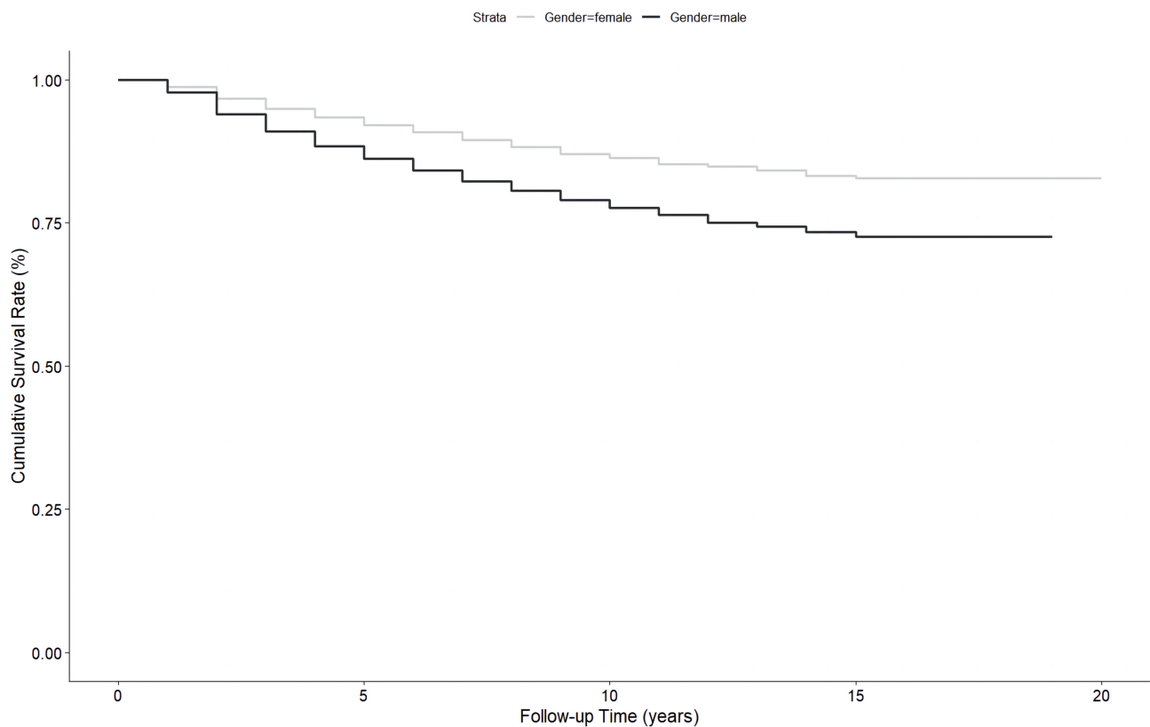
Figure 3 Cumulative Survival Probability of PLWH Receiving ART for Six Months and More by Sex in Sichuan Province, 2003–2022.
