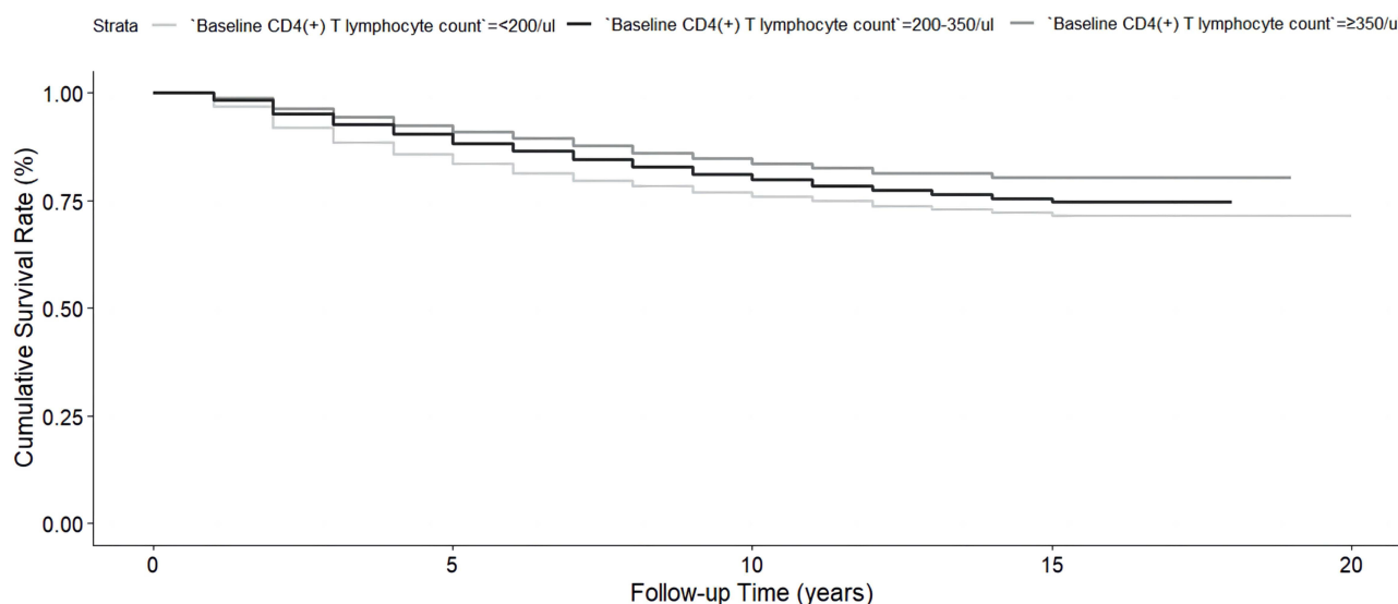
Figure 5 Cumulative survival probability of PLWH receiving ART for six months and more in different CD4(+) T cell level groups in Sichuan Province, 2003–2022.
