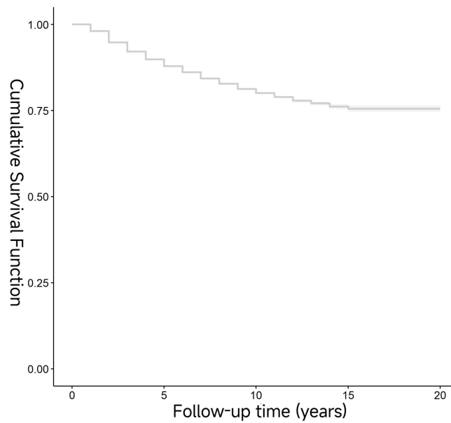
Figure 2 Cumulative Survival Probability of PLWH Receiving Antiviral Therapy for Six Months or More in Sichuan Province, 2003–2022.
