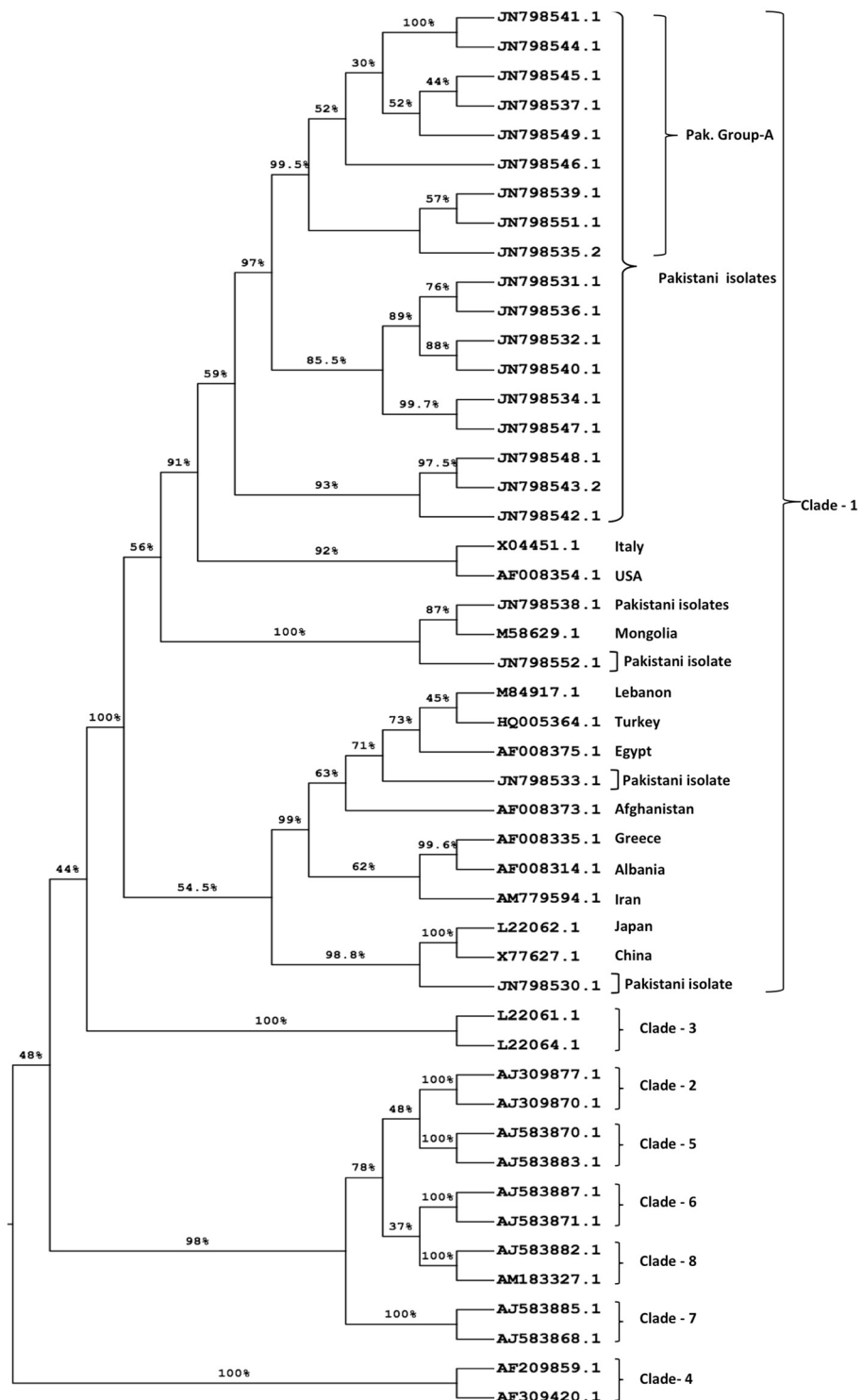
Figure 3 Phylogenetic Analysis of L-HDAg nucleotide sequences from position 856–1282 of isolates from Karachi, Pakistan and reference sequences obtained from GenBank. The analysis was carried out using Bayesian method by applying the Markov Chain Monte Carlo simulation using the software BEAST ver. 1.7.2. The values at the nodes of the tree show the posterior probabilities of the analysis.
