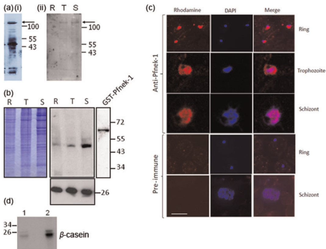
Fig. 1. Expression of Pfnek-1 in asexual parasites. (a) Western blot analysis detecting the full-length protein. Asynchronous (i, chicken antibody) or synchronous (ii, rabbit antibody) parasite extract (15 \mu g) was loaded on the gels. Arrows indicate the position of Pfnek-1. (b) Western blot analysis (rabbit antibody) showing that the antibody recognizes recombinant GST-Pfnek-1 (Dorin et al. , 2001) (far right lane) and displays a loading control (antibody against P. falciparum 2-Cys peroxiredoxin). R, Rings; T, trophozoites; S, schizonts. Molecular masses of co-migrating markers are indicated in kDa. (c) Immunofluorescence analysis. Synchronized asexual parasites were stained with the immunopurified rabbit anti-Pfnek-1 antibody (top panels). The two bottom panels display negative controls using pre-immune serum. Bar, 5 \mu m. (d) Immunoprecipitated kinase activity. The anti-Pfnek-1 rabbit antibody was used to immunoprecipitate \beta -casein kinase activity from 3D7 parasite extracts (lane 2). The pre-immune serum was used as a control (lane 1).
