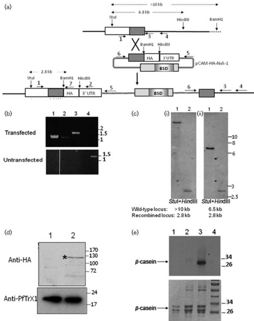
Fig. 3. HA tagging of the pfnek-1 locus. (a) Strategy for HA tagging. The locations of the primers used in PCR diagnostics are indicated with numbered arrows, and the positions of the restriction sites used for Southern blot analysis are shown. (b) PCR genotyping analysis. Genomic DNA was isolated from pCAM-HA- nek-1 -transfected parasites and from parental 3D7 parasites, and subjected to PCR using the indicated primers (see Fig. 3a). Lanes: 1, primers 1 + 7 (diagnostic for 5' integration event, 1.2 kb); 2, primers 6 + 3 (diagnostic for 3' integration event, 1.2 kb); 3, primers 6 + 4 (diagnostic for 3' integration event, 1.5 kb); 4, primers 1 + 4 (diagnostic for wild-type locus, 1.5 kb). Sizes of co-migrating markers are indicated in kb. (c) Southern blot analysis of transfected parasites. Total DNA digested with Stul and HindIII (i) or Stul and BamHI (ii) was probed with a fragment spanning nucleotides 577–1155 of the pfnek-1 coding region. Sizes of co-migrating markers are indicated in kb. (d) Western blot analysis of HA-tagged Pfnek-1. Protein extracts (15 \mu g) from the parental 3D7 wild-type clone (lane 1) and pCAM-HA- nek-1 -transfected parasites (lane 2) were probed with an anti-HA antibody. Sizes of co-migrating markers are indicated in kDa. (e) Anti-HA antibodies immunoprecipitate kinase activity from transfected parasites. Anti-HA antibodies were incubated with extracts from the parental 3D7 wild-type clone (lane 2) or pCAM-HA- Nek-1 -transfected parasites (lane 3). Immunoprecipitated material was assayed for \beta -casein activity. Lane 1 shows the kinase assay with \beta -casein alone (no immunoprecipitate added), and the molecular mass marker is shown in lane 4. Molecular masses are indicated in kDa.
