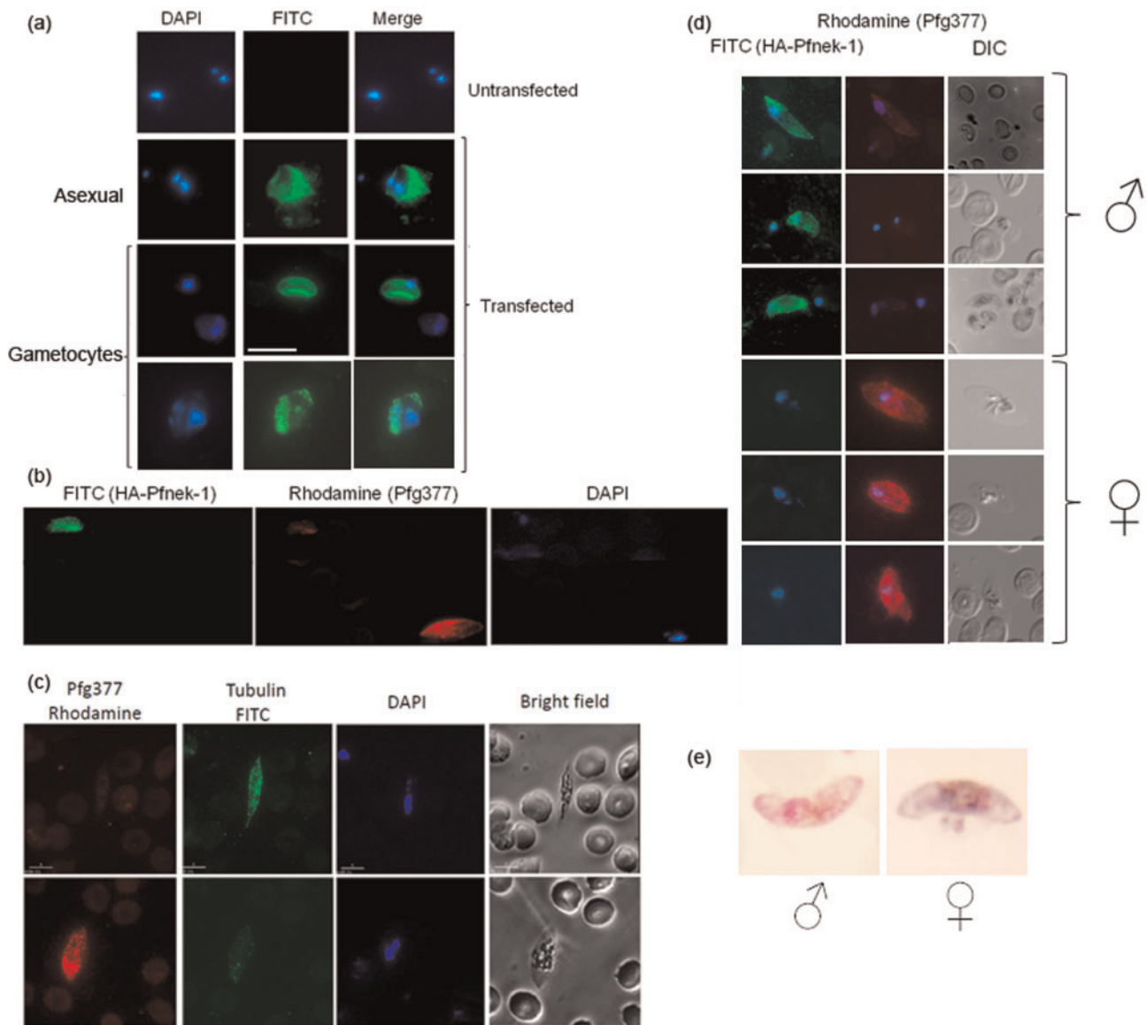
Fig. 4. Immunofluorescence analyses of male and female gametocytes. (a) Detection of HA-Pfnek-1 in asexual parasites (line 2) and gametocytes (lines 3 and 4) transfected with pCAM-HA-Nek-1 using an anti-HA antibody. The top line shows the negative control (staining of wild-type parasites with the anti-HA antibody). Bar, 10 \mu m. (b) A single microscopic field is presented, showing mutually exclusive staining with both antibodies. DAPI (blue), and anti-mouse-FITC (green) and anti-rat-rhodamine (red) secondary antibodies were used. (c) Tubulin is expressed predominantly in male gametocytes. Co-staining was performed with the \alpha -tubulin antibody and an antibody against Pfg377, a protein expressed predominantly in female gametocytes. (d) Further examples of the sex-specificity of HA-Pfnek-1 expression. (e) Typical images of Giemsa-stained stage V gametocytes, used to determine the sex ratio in Table 1. Bar, 10 \mu m. ♂, Male; ♀, female.
