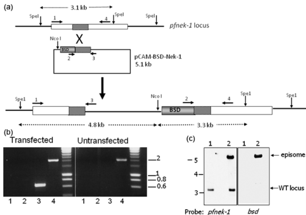
Fig. 2. Attempt to disrupt the pfnek-1 gene. (a) Strategy for pfnek-1 gene disruption. The knockout vector contains a PCR fragment spanning positions 73–630 of Pfnek-1 coding sequence, excluding two kinase subdomains essential for activity. Single crossover homologous recombination results in a pseudo-diploid configuration with two truncated copies lacking essential catalytic residues. The location of PCR primers (numbered arrows) and the restriction sites used for Southern blot analysis are indicated. (b) PCR genotyping. Genomic DNA was isolated from transfected and parental 3D7 parasites, and subjected to PCR using the indicated primers (see Fig. 2a). Lanes: 1, primers 1 + 3 (diagnostic for 5' integration event, 0.6 kb); 2, primers 2 + 4 (diagnostic for 3' integration event, 1.5 kb); 3, primers 2 + 3 (diagnostic for the episome, 0.7 kb); 4, primers 1 + 4 (diagnostic for wild-type locus, 2.1 kb). Sizes of co-migrating markers are indicated in kb. (c) Southern blot analysis of transfected parasites. Genomic DNA digested with SpeI and NcoI was probed with the Pfnek-1 fragment used in the pCAM-BSD-Nek-1 vector (positions 73 to 630 of the coding sequence). Sizes of co-migrating markers are indicated in kb.
