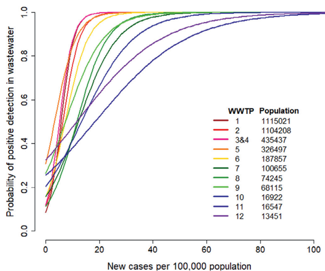
Fig. 1 – Probability of positive detection of SARS-CoV-2 RNA in wastewater versus the number of clinical diagnosed COVID-19 new cases per 100,000 population in each community served by corresponding WWTP.
