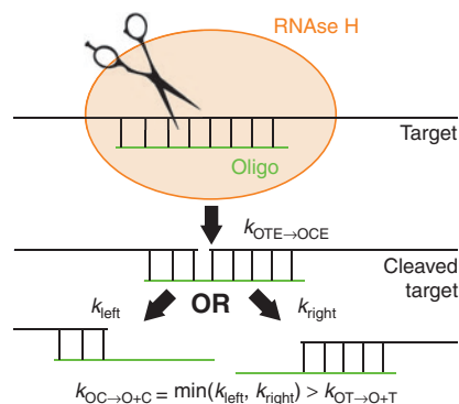
Figure 3 Schematic drawing of target cleavage illustrating the rationale for introducing the coupling k_{OT \rightarrow O+T} = -\alpha \cdot k_{OC \rightarrow O+C} . Upon enzyme (E, RNase H) binding to the OT complex the target is cleaved at a rate k_{OTE \rightarrow OCE} . After cleavage, the right and left parts of the cleaved target will dissociate from the oligonucleotide at (faster) rates k_{right} and k_{left} , respectively.
