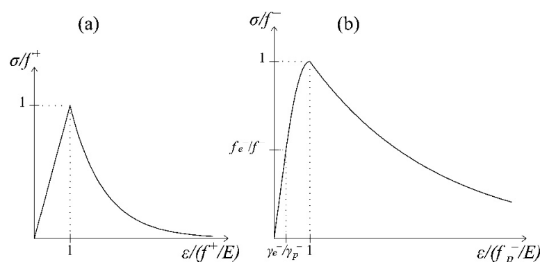
Figure 3. Uniaxial normalized \sigma - \epsilon curves: (a) softening behavior in tension and (b) in compression.
