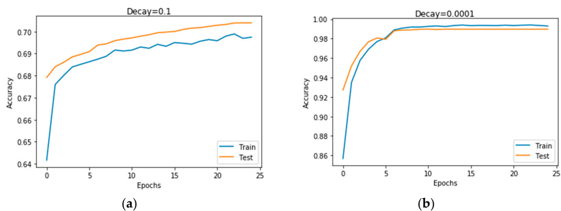
Figure 18. Recognition accuracy of the model with decay values of 0.1 and 0.0001. (a) shows that at higher value of 0.1 the model overfits whereas (b) shows that at lower values such as 0.0001, the system was able to generalize.
