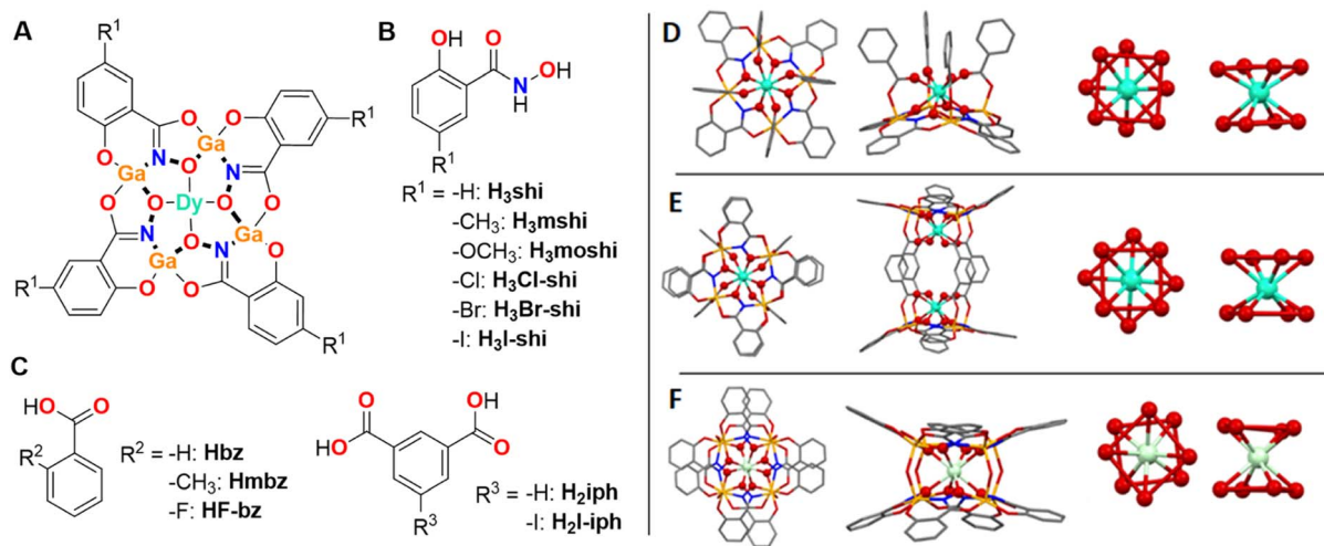
Fig. 1 (A) Schematic presentation of a \text{Dy}^{3+}[\text{12-MC}_{\text{GaN}}(\text{R}^1\text{-shi})\text{-4}] MC core, where \text{Ga}^{3+} and \text{R}^1 -substituted \text{H}_3\text{shi} (B) template the formation of the MC, while \text{Dy}^{3+} is linked to the central cavity by the derivatives of benzoic or isophthalic acids (C). (D–F) Top-down (left) and side-on (left-centre) views of the three \text{Ga}^{3+}/\text{Dy}^{3+} MCs geometries and the corresponding primary coordination spheres about \text{Dy}^{3+} (centre-left and right views, the red lines between oxygen atoms are guides for the eyes to suggest \text{O}_4 planes coming from the MC ring and otherwise). (D) [\text{DyGa}_4(\text{shi})_4(\text{bz})_4] representing the \text{LnM}_4(\text{L}')_4(\text{L}'')_4 structure (type A). 43 (E) [\text{Dy}_2\text{Ga}_8(\text{shi})_8(\text{iph})_4] corresponding to the \text{Ln}_2\text{M}_8(\text{L}')_8(\text{L}'')_4 structure (type B). 44 (F) [\text{DyGa}_8(\text{shi})_8(\text{OH})_4] corresponding to the \text{LnM}_8(\text{L}')_8(\text{OH})_4 structure (type C). 45 The structure was solved for isostructural [\text{NdGa}_8(\text{shi})_8(\text{OH})_4]\text{Na} . Solvents of crystallization, counter ions, and hydrogen atoms are omitted for clarity. Central \text{Ln}^{3+} and coordinating oxygen atoms are bolded for highlight effect. Colour code: Ga, orange; Ln, teal; O, red; N, blue; C, grey.
