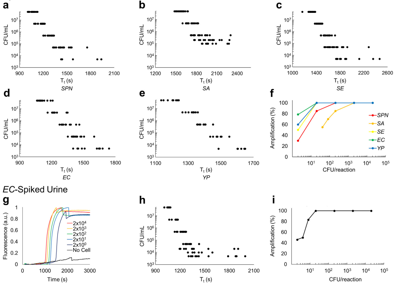
Fig. 4. SmarT-LAMP quantitation of diverse pathogens in spiked murine whole blood and human donor urine. (a–e) T_t values for SPN, SE, EC, YP ( 2 – 2 \times 10^4 CFU/reaction); SA ( 4 \times 10^1 – 2 \times 10^4 CFU/reaction). (f) Percentage of total pathogen samples amplifying at each concentration in smarT-LAMP. (g, h) Representative traces and T_t values for EC in spiked human donor urine ( 2 – 2 \times 10^4 CFU/reaction). (i) Percentage of total EC samples amplifying at each concentration in smarT-LAMP ( \geq 10 samples/concentration).
