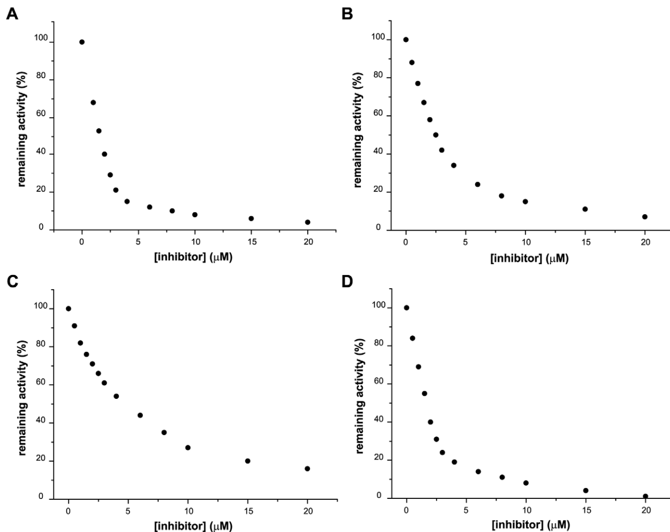
Figure 4. Inhibition of TR activity of TGR by active compounds. Remaining TR activity as a function of inhibitor concentration is plotted for a. 1 , b. 2 , c. 3 and d. 50 . 1 nM TGR was used in all assays. doi:10.1371/journal.pone.0035033.g004
