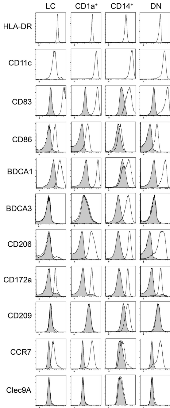
Figure 4. Phenotype of migratory skin DC subsets. Cells isolated after skin explant culture were stained for HLA-DR, CD11c, CD1a, CD14, EpCAM, BDCA1, Clec9A, CD206, CD83, CD86, BDCA3, CD172a, CD209, CCR7, or control isotype. Representative results of five independent experiments are shown.
