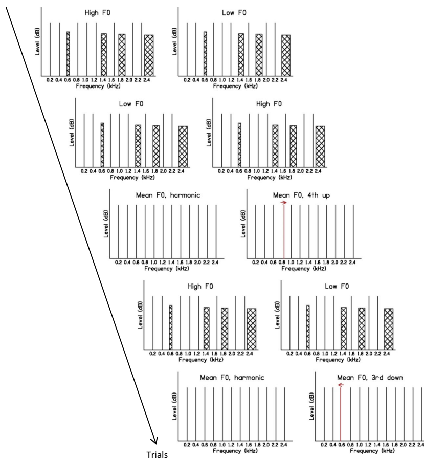
FIG. 1. Schematic diagram of a possible trial sequence for condition UNREL3. In context trials, harmonic 3 plus harmonics 7, 9, and 12 are replaced by non-informative noise bands. The difference in F0 between the low and the high cases can be most easily seen by comparing the positions of the high harmonics to the fixed position of the noise bands. Trial 1: context trial with higher F0
