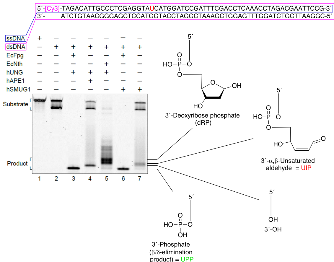
Figure 7. Indirect identification of UIP by electrophoretic mobility without exposure of DNA to high temperature. U-DNA (substrate 1, 1 pmol) was incubated with hSMUG1 (0.3 pmol) at 37°C for 30 min; either alone or together with EcFpg (4 pmol) as indicated. To define the different 3'-end products, substrate was incubated with hUNG (1 pmol) together with either EcFpg (4 pmol), hAPE1 (0.45 pmol) or EcNth (1 pmol), as indicated, under the same conditions. Incubations were also performed with either substrate 1 (dsDNA; lane 2) or the labelled strand of substrate 1 (ssDNA; lane 1) alone, showing that the upper substrate band is ssDNA and the lower band dsDNA. Incision product was separated from un-incised DNA by PAGE at 300 V for 5 h using a 20% (w/v) gel with 7 M urea.
