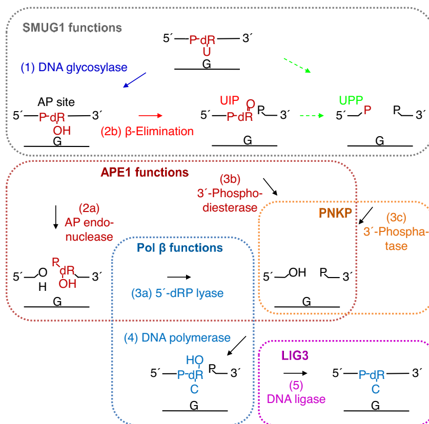
Figure 10. Proposed steps in the human BER pathway after SMUG1 has targeted uracil in DNA. After uracil has been removed by the DNA glycosylase activity of SMUG1 (step 1; blue), the latter is either replaced by APE1 (dark red) which incises the AP site (step 2a), or SMUG1 itself incises the AP site (step 2b; red) leaving behind a 3'- \alpha,\beta -unsaturated aldehyde (UIP) which can be removed by APE1 (step 3b). Further processing of UIP (or maybe an alternative type of incision of the AP site; green broken arrows) results in a 3'-phosphate (UPP) which is a substrate for PNKP (orange). The cleaned one nucleotide gap in DNA is now ready for insertion of the correct dCMP (step 4) by the repair DNA polymerase \beta (Pol \beta ; dark blue), which also exhibits the dRP lyase activity which removes the 5'-dRP remnant (step 3a) after APE1 incision. BER is concluded by nick-sealing (step 5) by DNA ligase III (LIG3; purple). The residues removed are indicated in dark red; those resulting from replacement in dark blue; dR, deoxyribose.
