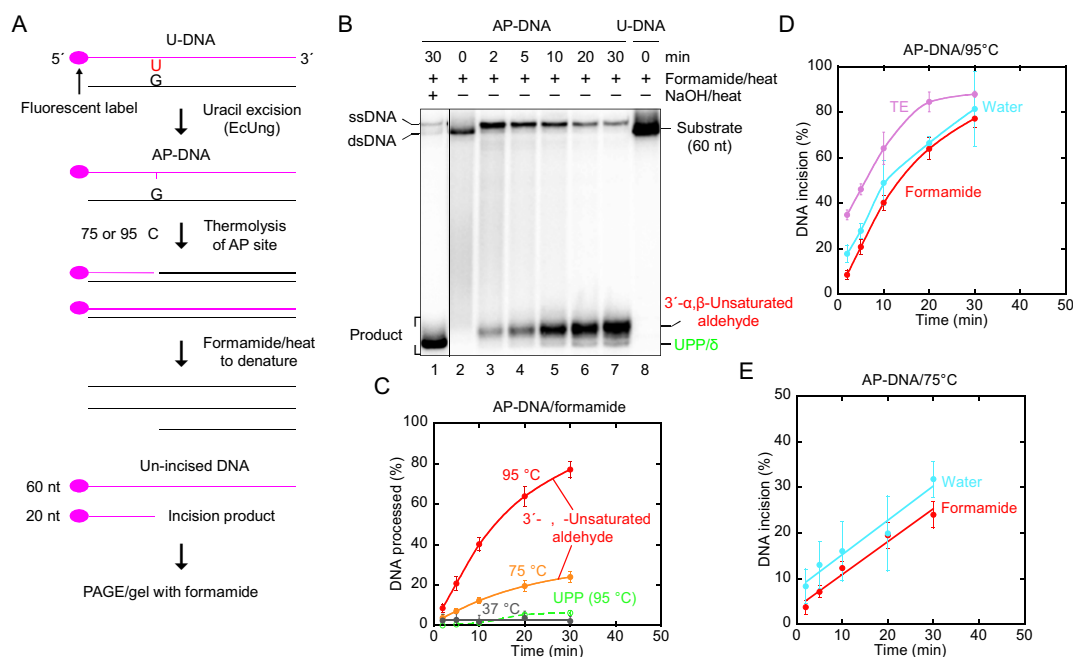
Figure 2. Thermolysis of AP-DNA at high temperature efficiently forms UIP as opposed to UPP. (A) DNA substrate (see below) and assay. (B) Time dependence for cleavage of AP-DNA at 95°C. AP-DNA derived from substrate 1 (0.5 pmol) was treated with loading solution used in conventional denaturing PAGE [containing 80% (v/v) formamide]. UIP forms efficiently, while a smaller amount of UPP/ \delta -product appears at the longest incubation times. (C) Time dependence for cleavage of AP-DNA at different temperatures. AP-DNA derived from substrate 1 was used at 37°C (1 pmol) and 95°C (see B), while that used at 75°C (1 pmol) was derived from substrate 2 (see Materials and Methods). Each value represents the average ( \pm SD) of 6–15 (95°C; red), 2–6 (75°C; orange) or 5–6 (37°C; dark grey) independent measurements. At 37°C, PAGE was performed on a 15% (w/v) gel containing 3% (v/v) formamide, and identical experiments with AP-DNA dissolved in pure water also showed no significant DNA cleavage (data not shown). UPP (green) was only formed at 95°C. (D) Time dependence for AP-DNA cleavage in different solutions at 95°C. Treatment in loading solution (red; described in B), water (blue) or TE buffer (violet) showed that the initial cleavage of AP-DNA is virtually identical in the different aqueous solutions. To separate incised DNA from un-incised DNA the reaction products were subjected to denaturing (red) or non-denaturing (blue; violet) PAGE. Each value represents the average ( \pm SD) of 4–17 independent measurements, where the slopes of the graphs for the initial DNA incision, i.e. the first three data points (6–17 independent measurements; red, y = 3.95x + 0.769 , R = 0.999 ; blue, y = 3.92x + 9.29 , R = 0.998 ; violet, y = 3.65x + 27.673 , R = 0.999 ) yield the non-enzymatic incision per min. This amounted to 3.95% of the AP sites incised per min, resulting in a background of 19.8% non-enzymatic hydrolysis (as calculated from the red graph; for the 5 min formamide/heat treatment) for the experiment described in Figure 1B and C. The amount of background incision was subtracted giving the value for enzymatic U-DNA incision for all experiments using 5 min heat treatment at 95°C (Figure 1C). (E) Time dependence for AP-DNA cleavage in different solutions at 75°C. AP-DNA (substrate 2, 1 pmol) was exposed to loading solution (red) or water (blue). Each value represents the average ( \pm SD) of 6 (at 2–20 min) or 2–3 (at 30 min) independent measurements. To separate incised DNA from un-incised DNA the reaction products were subjected to denaturing (red) or non-denaturing (blue) PAGE. The initial slopes of the graphs (red, y = 0.722x + 3.65 , R = 0.986 ; blue, y = 0.755x + 7.68 , R = 0.977 ) yield the non-enzymatic incision per min. This amounted to 0.722% of the AP sites incised per min in the formamide solution. Abbreviation: \delta , \beta/\delta -elimination product.
