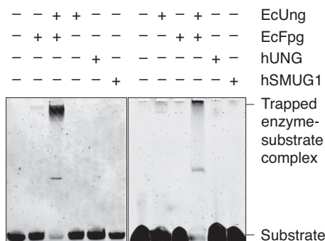
Figure 6. Trapping experiments for Schiff base intermediate. Left panel, EcFpg (17 pmol) alone as a negative control, and together with EcUng (3 pmol) as a positive control, EcUng as well as hUNG (5 pmol) alone as negative controls, and hSMUG1 (0.3 pmol) alone, were incubated with substrate 2 (1 pmol) and 50 mM NaBH 4 in reaction buffer at 37°C for 1 h (final volume, 10 \mu l). Right panel, EcFpg (10 pmol) alone as a negative control, and together with EcUng (10 pmol) as a positive control, EcUng as well as hUNG (10 pmol) alone as negative controls, and hSMUG1 (10 pmol) alone, were incubated with substrate 2 (1 pmol) and 50 mM NaBH 4 in reaction buffer at 37°C for 1 h (final volume, 10 \mu l). In each case (A and B), trapped was separated from un-trapped substrate by denaturing PAGE [10% (w/v)] at 200 V for 1 h. The experiments were performed in triplicate showing the same result.
