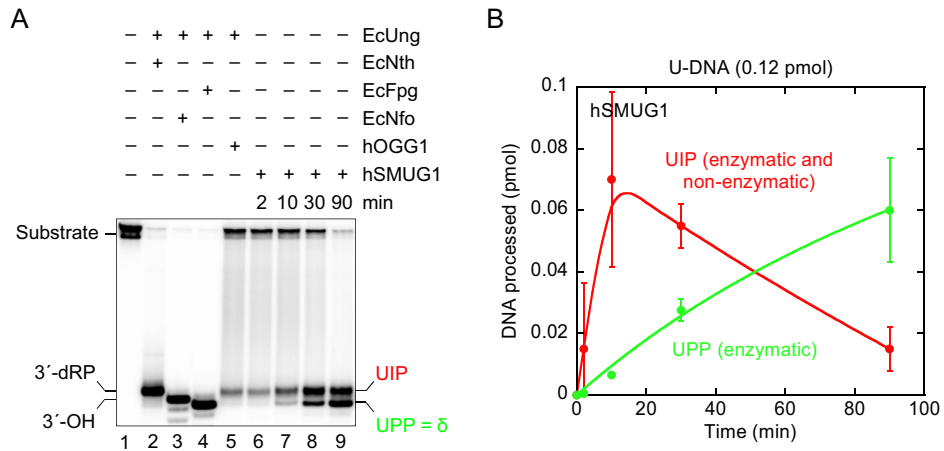
Figure 3. Indirect identification of UIP and UPP by electrophoretic mobility using conventional denaturing conditions. (A, B) Time dependence of UIP (red) and UPP (green) formation by hSMUG1. hSMUG1 (0.3 pmol) was incubated with substrate 1 [ 32 P] (0.12 pmol) in 20 mM Tris-HCl, pH 8.0, 1 mM DTT, 1 mM EDTA, 70 mM KCl at 37°C. To define the different 3'-end products, substrate was incubated with either EcNth (8.7 pmol), EcNfo (0.16 pmol), EcFpg (17 pmol) or hOGG1 (13 pmol) together with EcUng (0.78 pmol) for 10 min. Incised was separated from un-incised DNA by denaturing PAGE. Each value in B represents the average (±SD) of three independent measurements.
