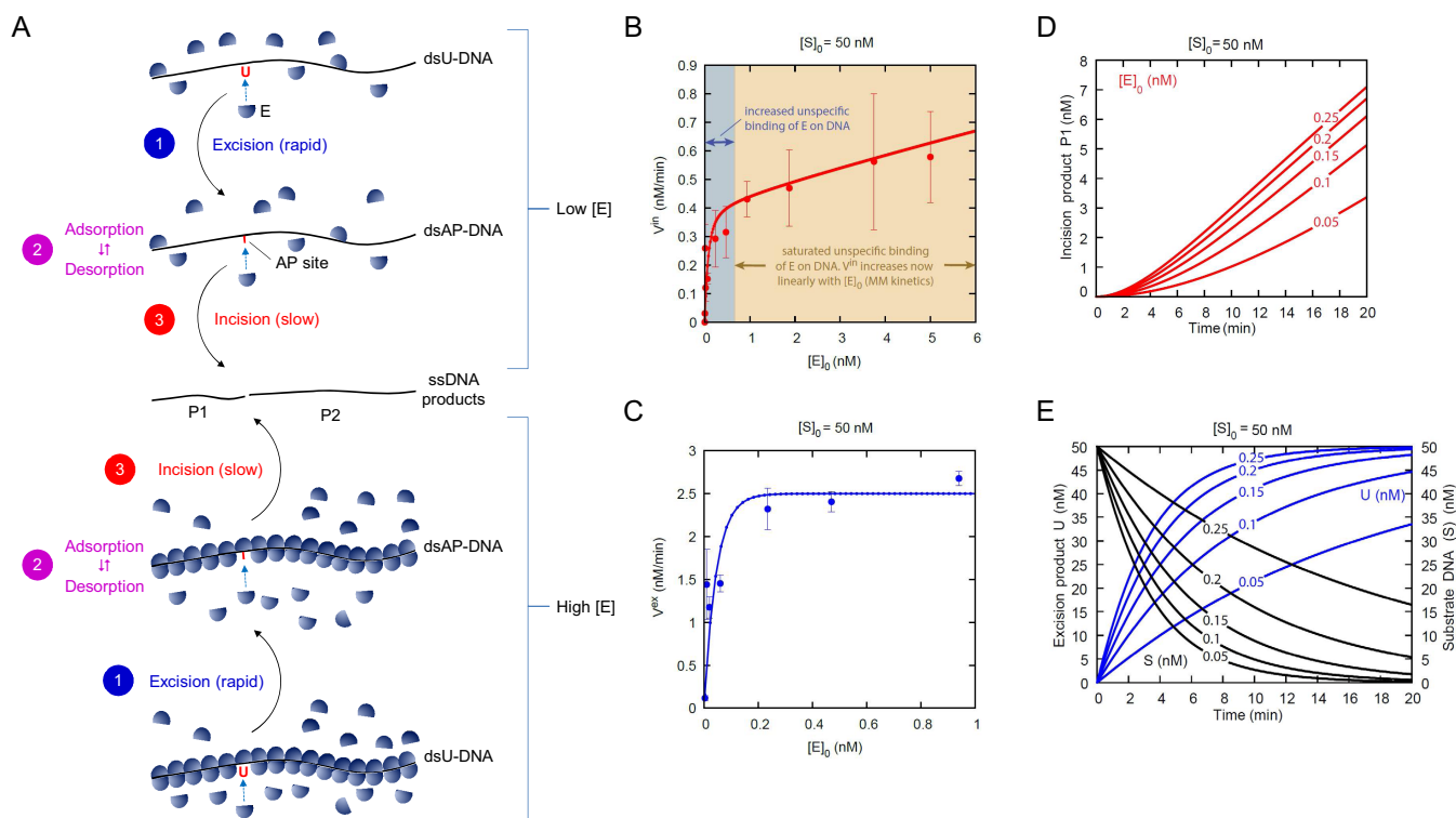
Figure 9. hSMUG1 kinetics. (A) Three-phase kinetic model. Phase 1 is shown in blue, phase 2 in violet and phase 3 in red. The uracil excision step is rapid compared to the slow DNA incision step. (B) U-DNA incision rate V^{in} and (C) uracil excision rate V^{ex} (see A) as a function of enzyme concentration [E]_0 at an initial U-DNA concentration [S]_0 of 50 nM, where the corresponding time-dependent data in the range [E]_0 = 0.05 –0.25 nM (red line) is presented in (D) showing that at higher initial enzyme (E) concentration the model predicts that the formation of the incision product P1 has linear time-dependent kinetics, and in (E), showing that the excision kinetics for U (blue line) are fast and correlate with the removal of substrate DNA (S; black line), respectively. Incubation was performed for 20 min as described in Figure 4B. The V^{in} in the blue area changes as a result of increased unspecific binding of enzyme to DNA. In the yellow area, the unspecific binding is saturated and the V^{in} follows Michaelis–Menten (MM) kinetics. Each value represents the average ( \pm SD) of 3–6 independent measurements.
