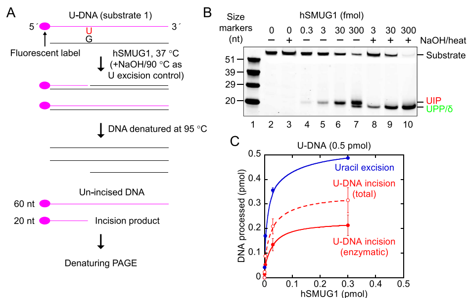
Figure 1. Indication of hSMUG1 incision at uracil in DNA. (A) DNA substrate and conventional base excision assay. (B, C) Protein dependence of U-DNA incision (red) and uracil excision (blue). hSMUG1 was incubated with U-DNA (substrate 1, 0.5 pmol) in 20 mM Tris-HCl, pH 8.0, 1 mM DTT, 1 mM EDTA, 70 mM KCl at 37°C for 10 min. Each value in C represents the average ( \pm SD) of three independent measurements. 'U-DNA incision (total)' corresponds to the values obtained from measuring the strength of the bands on the gel in B (lanes 4–7); the 'U-DNA incision (enzymatic)' values are calculated by subtracting the amount of AP site incision caused by the 5-min heat treatment at 95°C (as presented in Figure 2D) from the 'U-DNA incision (total)' values, where the number of AP sites formed by hSMUG1 equals the number of uracils excised as measured in parallel in B (lanes 8–10). Abbreviation: nt, nucleotides; UIP, U-DNA incision product; UPP, U-DNA processing product.
