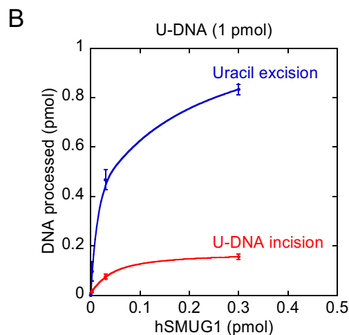
Figure 5. hSMUG1 incises at uracil in ssDNA. (A, B) Protein dependence of U-DNA incision (red) and uracil excision (blue). hSMUG1 was incubated with ssU-DNA (1 pmol; the labelled strand of substrate 1) at 37°C for 10 min. Each value in B represents the average of 2 independent measurements. Incision product was separated from un-incised DNA by PAGE at 100 V for 50 min using a 12% (w/v) gel with 3% (v/v) formamide.
