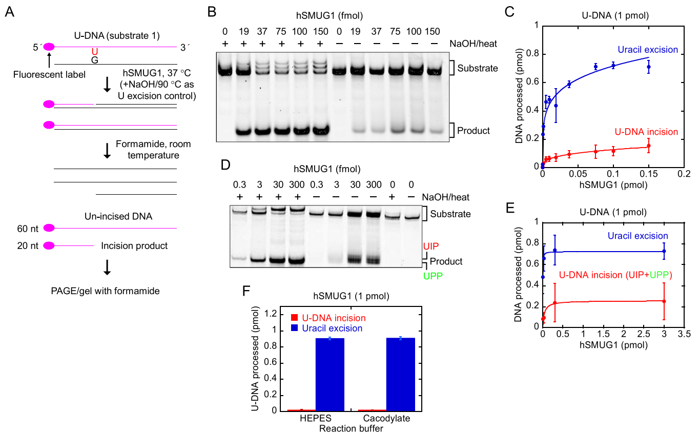
Figure 4. hSMUG1 incises at uracil in DNA. (A) DNA substrate and assay. (B, C) Protein dependence of U-DNA incision (red) and uracil excision (blue). hSMUG1 was incubated with U-DNA (substrate 1, 1 pmol) at 37°C for 10 min. Each value in C represents the average (±SD) of 3–6 independent measurements. Incision product was separated from un-incised DNA by PAGE at 115 V for 1.5 h using a 20% (w/v) gel with 3% (v/v) formamide. (D) hSMUG1(25–270) was incubated with U-DNA (1 pmol of substrate 1; see A) at 37°C for 20 min. Incision product was separated from un-incised DNA by PAGE at 120 V for 2 h using a 20% (w/v) gel with 3% (v/v) formamide. (E) Protein dependence of U-DNA incision/processing (red) and uracil excision (blue). Each value represents the average (±SD) of 4–5 independent measurements as described in D. (F) U-DNA incision by hSMUG1 in different buffers. U-DNA (1 pmol of substrate 1) was incubated with 1 pmol of hSMUG1(25–270) or without enzyme as control in reaction buffer (HEPES), or in 45 mM sodium cacodylate with the same pH and additions as for reaction buffer (see Materials and Methods), at 37°C for 10 min (final volume, 20 μl). Incision product was separated from un-incised DNA by PAGE as described in E. Each value represents the average (±SD) of three independent measurements.
