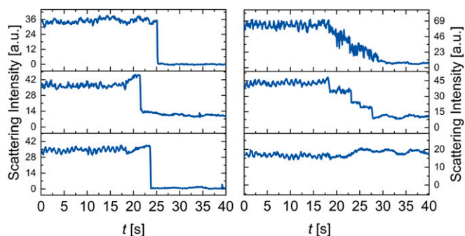
Fig. 3. Scattering emission of individual DOPG vesicles. Six representative scattering intensity profiles (after subtraction of background) of single DOPG vesicles upon exposure to 10 nM \alpha -synuclein at t = 0 . Difference in absolute scattering intensities between these data and Fig. 2B and SI Appendix, Figs. S4–S8 is due to differences in light intensity, chip variations, and image acquisition time. Intensity profiles were obtained using unlabeled vesicles.
