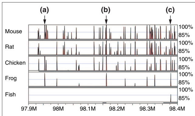
Figure 2 Interspecies comparison produced by the VISTA server [37,38], highlighting conserved elements. The conservation profiles were obtained with the human sequence as reference (chromosome 6, human genome build 34, megabase coordinates as indicated on the horizontal axis, in an intergenic region). The percentage identity was computed in sliding 100 bp windows by comparison with five different species. Frog is Xenopus tropicalis , and fish is Fugu rubripes . Arrows indicate: (a) an element conserved in mouse, frog and chicken, but not in rat; (b) ultraconserved element uc.196 [14] (221 bp, 100% conserved in mouse and rat); (c) an element conserved in all five species down to fish. The somewhat arbitrary conservation relationships (for example, a segment highly conserved between human and frog but not found in rat) is indicative of a stochastic process, in line with notions embodied in Figures 4 and 5.
