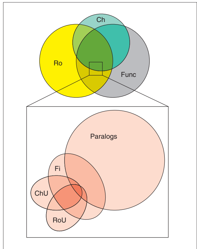
Figure 3 Overlap between different ANCOR sets. The quantitative relations are illustrative. The highlighted square zooms in on rare ANCORS, which are predicted to be functional. Ro, top 5% of conserved elements in a human-rodent comparison; Ch, the approximately 2.5% of the human genome that can be reliably aligned with chicken [18]; Func, the 5% portion of the human genome estimated to be functional on the basis of rodent comparisons [10,15]. Paralogs, noncoding sequences which belong to paralogous families within human genome [21]; Fi, elements conserved in the pufferfish Fugu rubripes genome [20]; RoU, ultraconserved elements, defined as > 200bp of 100% identity between human, mouse and rat [14]; ChU, the same definition for ultraconserved elements applied to human-chicken comparison [18].
