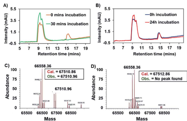
Fig. 5 (A) HPLC chromatograms of complex 7 (100 μM) and HSA (600 μM) pre- and post-incubation. (B) HPLC chromatogram of complex 8 (100 μM) and HSA (600 μM) pre- and post-incubation. (C) Deconvolved mass-spectrum of HSA (60 μM) incubated with complex 7 (180 μM) for 2 h. (D) Deconvolved mass-spectrum of HSA (60 μM) incubated with complex 8 (180 μM) for 2 h.
