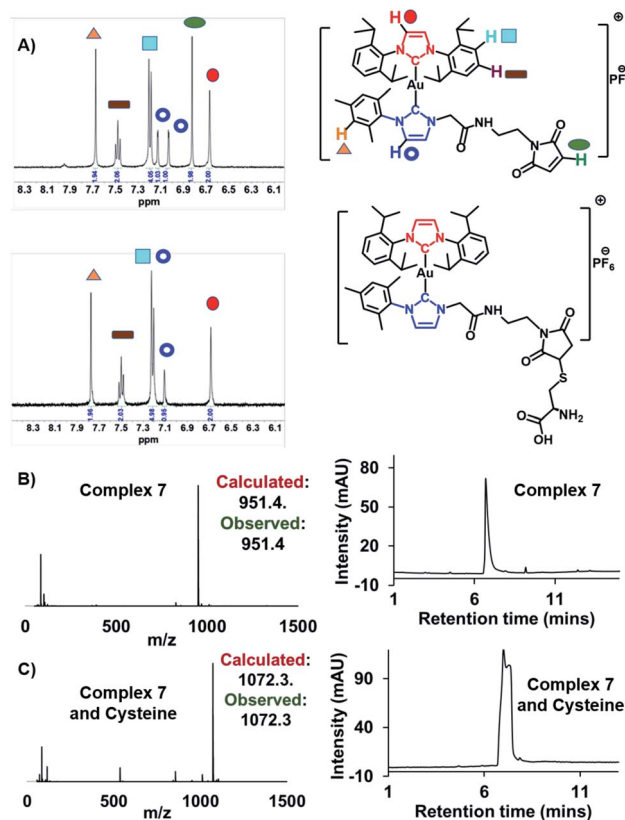
Fig. 4 (A) Change in the ^1\text{H} NMR spectrum in the aromatic region of complex 7 (2.25 mM) seen upon addition of 5 equivalents of cysteine in DMSO- d 6 /D 2 O (3 : 1) after 30 min at 37 °C. Please see the ESI† for the full spectrum. (B) Mass-spectrometric data and HPLC chromatogram corresponding to complex 7. (C) Mass-spectrometric data and HPLC chromatogram of complex 7 post-incubation with cysteine (5 equiv.).
