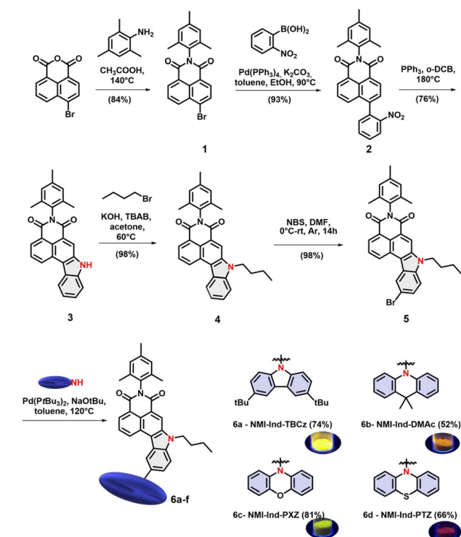
Scheme 1 The synthetic path towards “bow-like” TADF dyes 6a–d and their solid-state emission.
