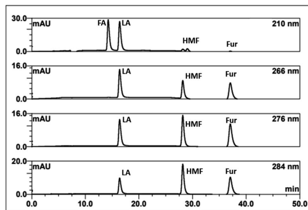
Fig. 2 HPLC-DAD chromatograms of the separation of FA, LA, HMF, furfural (Fur) through an \text{H}^+ ion exchange column with 0.1% TFA at 60 °C using detection at 210, 266, 276, and 284 nm.
