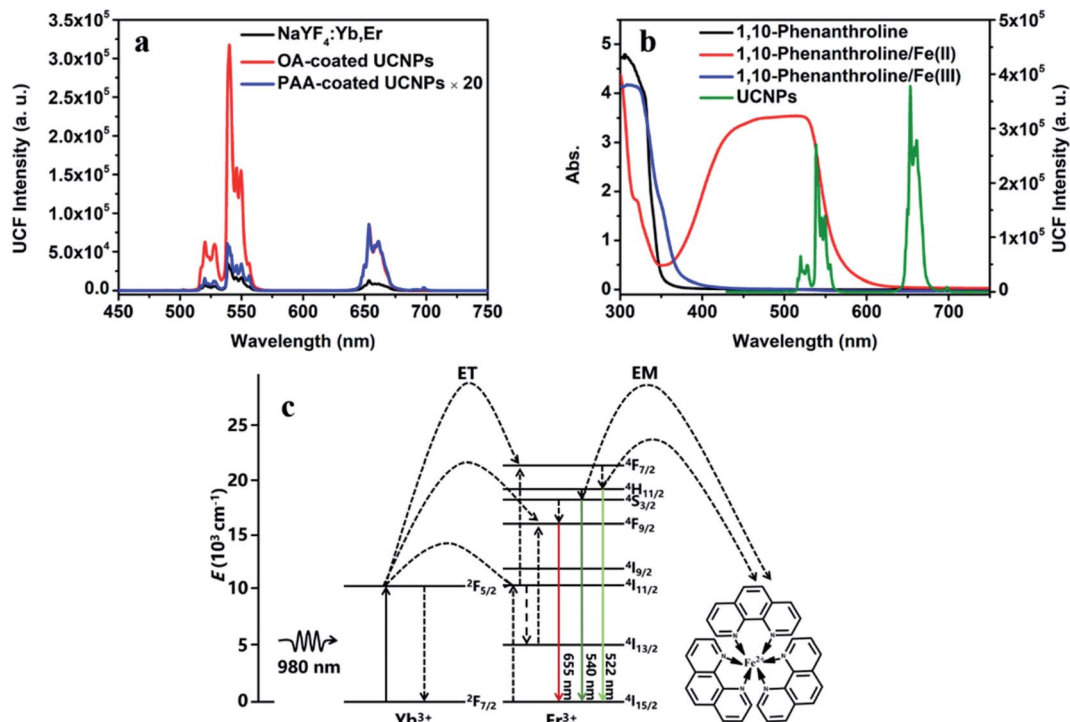
Fig. 2 (a) The upconversion emission spectrum of OA-coated core UCNPs (black line), OA-coated core-shell UCNPs (red line) and PAA-coated UCNPs (blue line). (b) Absorption spectrum of 1,10-phenanthroline ( 2.0 \text{ mmol L}^{-1} ) (black line), 1,10-phenanthroline ( 2.0 \text{ mmol L}^{-1} )/Fe(II) ( 0.4 \text{ mmol L}^{-1} ) (red line) and 1,10-phenanthroline ( 2.0 \text{ mmol L}^{-1} )/Fe(III) ( 0.4 \text{ mmol L}^{-1} ) (blue line). The upconversion emission spectrum of PAA-coated UCNPs (green line). (c) Proposed excitation and IFE mechanism in UCNPs/Fe(II)-1,10-phenanthroline system. [1,10-phenanthroline] = 2.0 \text{ mmol L}^{-1} , [Fe(II)] = 0.4 \text{ mmol L}^{-1} , [Fe(III)] = 0.4 \text{ mmol L}^{-1} .
