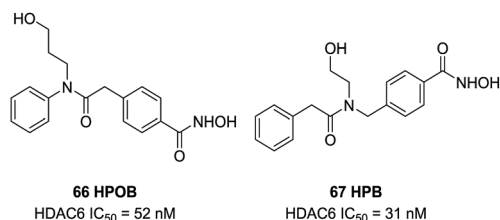
Fig. 28 Structures of branched linker based HDAC6 inhibitors.
