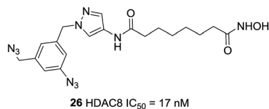
Fig. 10 Structures of pyrazole-based HDAC8 inhibitors.
