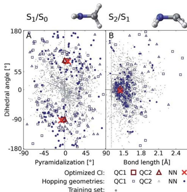
Fig. 6 Scatter plots showing the distribution of hopping geometries obtained with QC1, QC2, and NN as well as optimized S_1/S_0 (A) and S_2/S_1 (B) minimum energy conical intersections (CIs) along with the geometries that make up the training set with 4000 data points. The actual geometry is depicted on top (geometrical parameters are given in Fig. S7B†). A zoom-in of the regions near the optimized points is shown in Fig. S7A in the ESI† together with a definition of the dihedral and pyramidalization angles.
