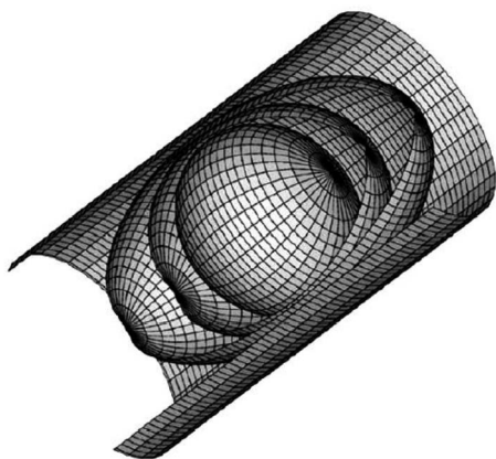
Fig. 13 Evolution of the ellipsoidal surface during powder compaction. 93
