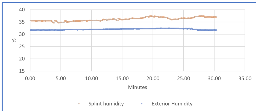
Figure 16. Humidity graph.
