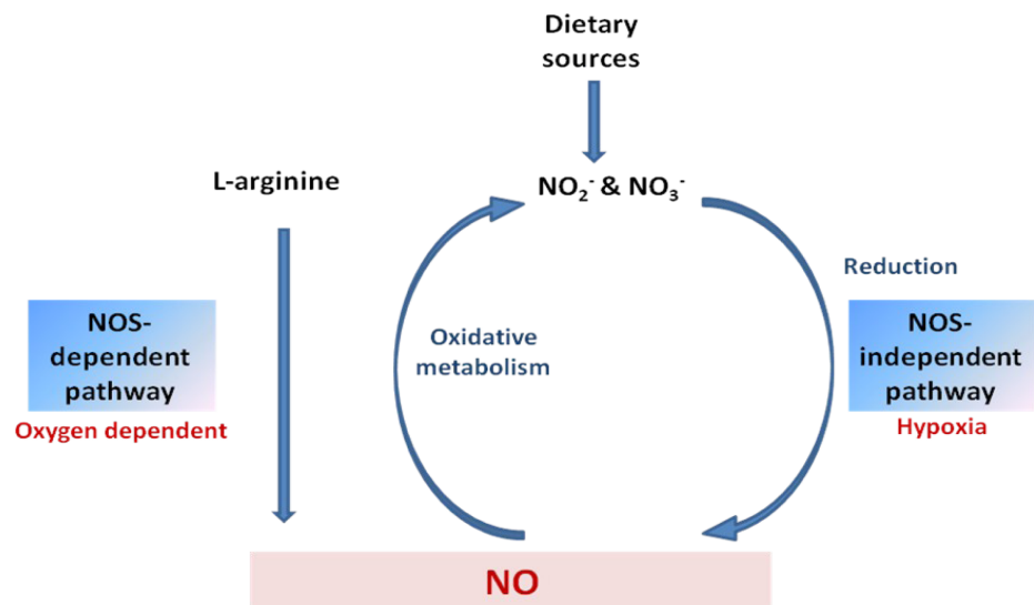
Figure 2. Nitric oxide, nitrite, and nitrate cycle.
