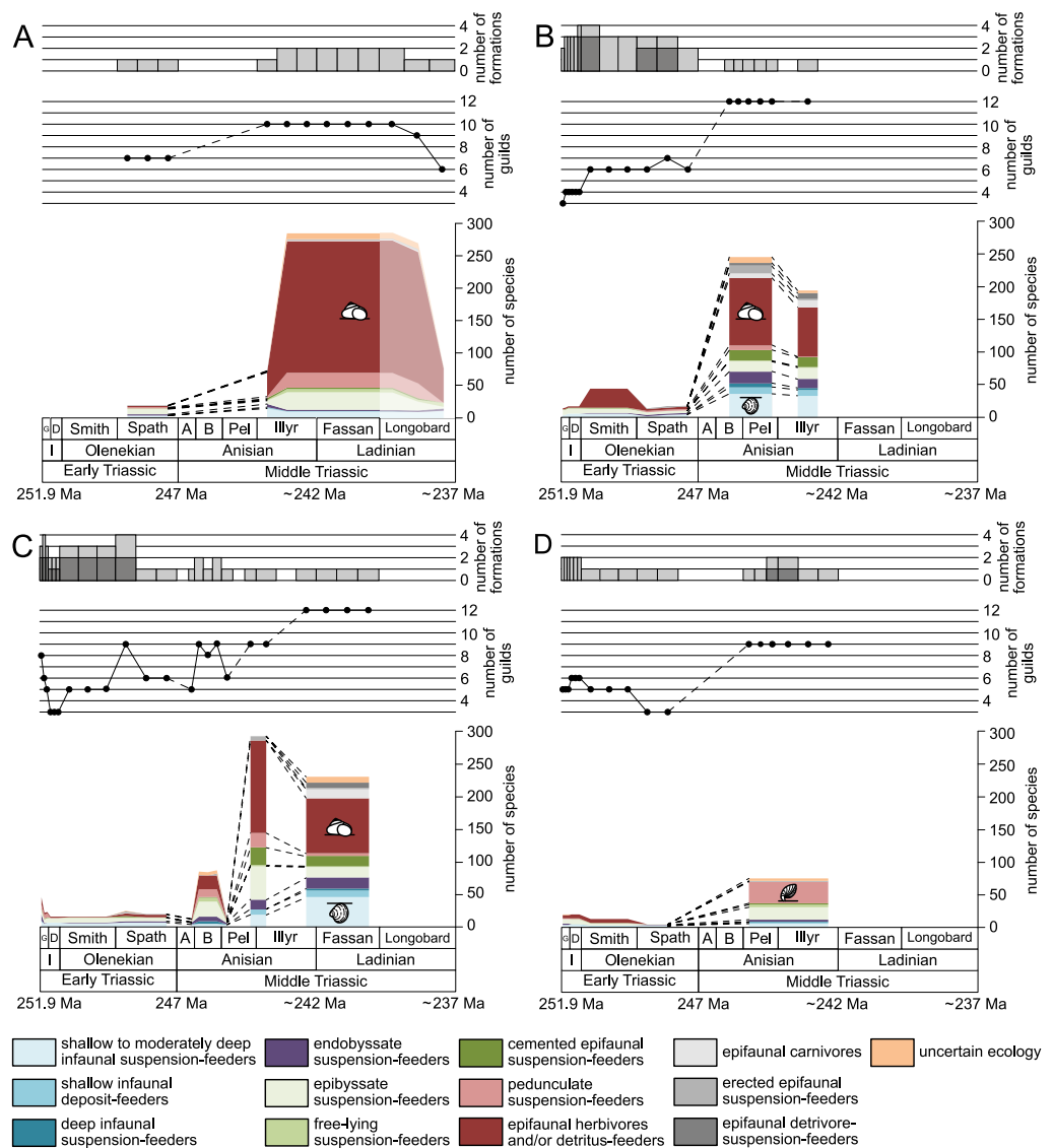
Figure 2 Maximum species richness in different environments. (A) lagoons, (B) inner ramps, (C) mid-ramps and (D) outer ramps. The Longobardian is palish to indicate that the decrease of species richness is not a primary signal. Light grey bars on top indicate the number of lithological units representing each time interval. In cases where information does not come from all lithological units representing the corresponding time interval, the actual number of lithological units from which information comes from is indicated by dark grey bars. Due to our data selection, the following guilds are not shown in this figure although reported in polished slabs: shallow infaunal deposit-feeders in late Griesbachian-Smithian and middle Spathian inner ramps (one species, respectively) and Smithian mid-ramps (one species), cemented epifaunal suspension-feeders in early-middle Spathian inner ramps (one species) and Dienerian-Smithian outer ramps (two species), epifaunal herbivores and/or detritus-feeders in early-middle Spathian (two species) and late Pelsonian-early Illyrian (five species) outer ramps. Abbreviations: Spath, Spathian. Further abbreviations, symbols for ecological guilds and information about the relative duration of substages as in Fig. 1. See text for further explanation.
