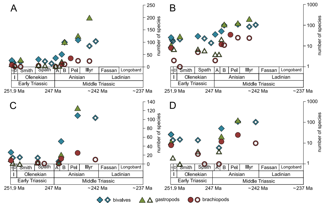
Figure 7 Maximum species richness of bivalves, gastropods and brachiopods throughout the Early and Middle Triassic. (A–B) in general and (C–D) in mid-ramps. Number of species illustrated with linear scale (A and C) and logarithmic scale (B and D). Filled symbols represent faunas that are more or as diverse as older ones, whereas empty symbols represent faunas that are less diverse than older ones. Abbreviations as in Fig. 1 and Fig. 2. Information about the relative duration of substages as in Fig. 1. See text for further explanation.
