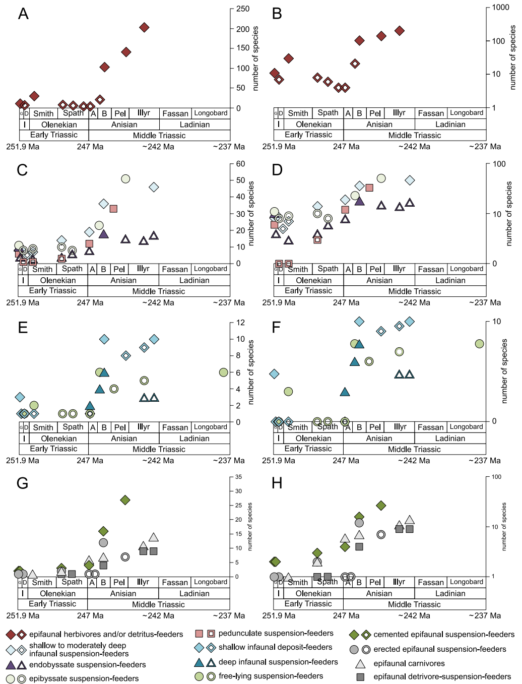
Figure 5 Maximum species richness throughout the Early and Middle Triassic of ecological guilds.
