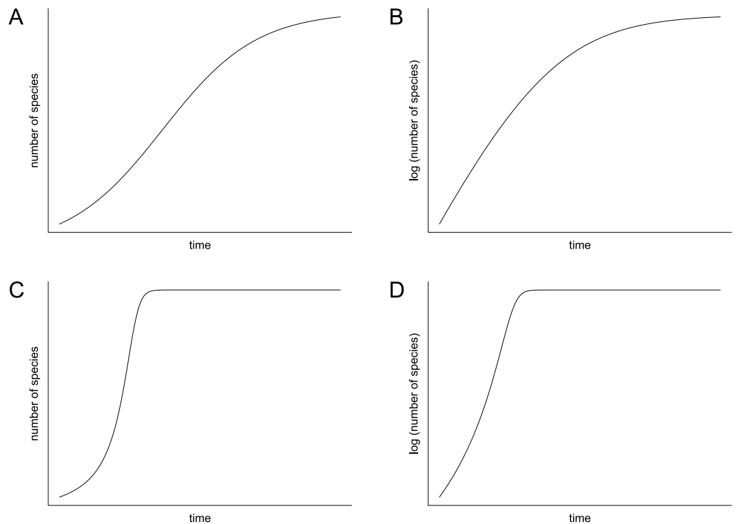
Figure 8 Diversification curves. (A–B) Logistic with number of species illustrated with linear scale (A) and logarithmic scale (B). (C–D) Hyperbolic-damped with number of species illustrated with linear scale (C) and logarithmic scale (D).
