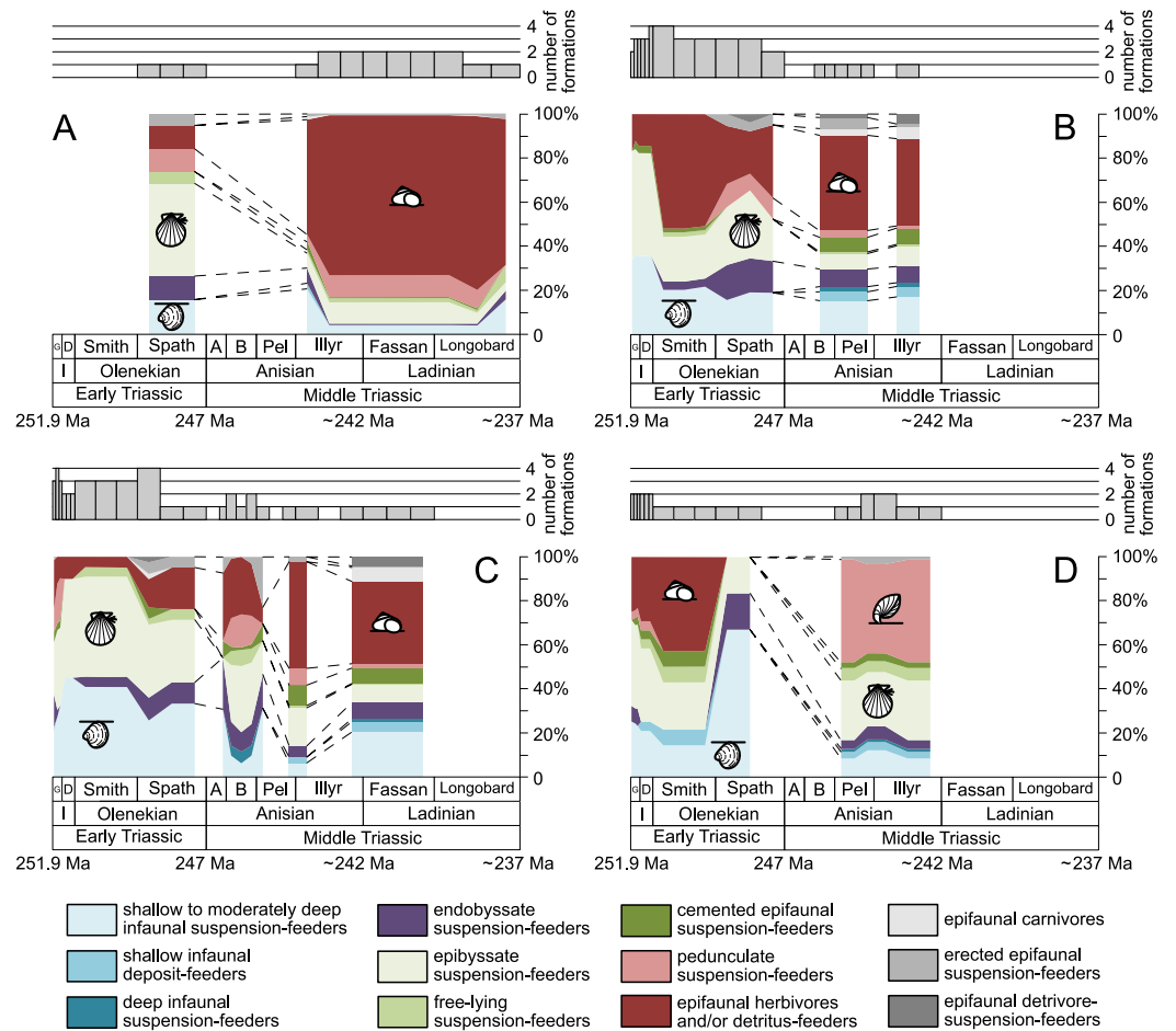
Figure 4 Guild-species diversity of different environments. (A) lagoons, (B) inner ramps, (C) mid-ramps and (D) outer ramps. Bars on top indicate the number of lithological units representing each time interval. Due to our data selection, the following guilds are not shown in this figure although reported in polished slabs: shallow infaunal deposit-feeders in late Griesbachian-Smithian and middle Spathian inner ramps (one species, respectively) and Smithian mid-ramps (one species), cemented epifaunal suspension-feeders in early-middle Spathian inner ramps (one species) and Dienerian-Smithian outer ramps (two species), epifaunal herbivores and/or detritus-feeders in early-middle Spathian (two species) and late Pelsonian-early Illyrian (five species) outer ramps. Abbreviations as in Figs. 1 and 2. Symbols for ecological guilds and information about the relative duration of substages as in Fig. 1. See text for further explanation.
