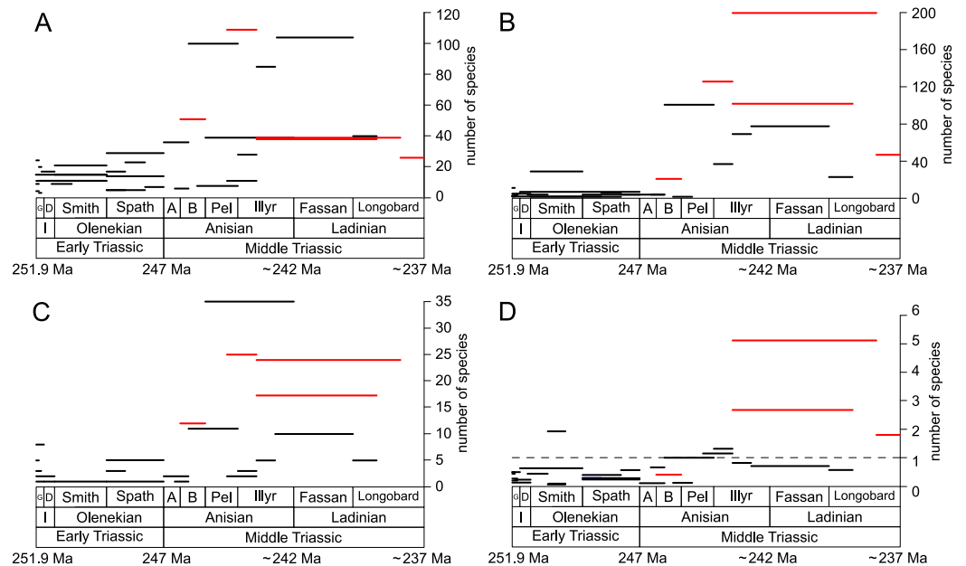
Figure 6 Species richness of the most diverse taxa and the gastropod/bivalve-ratio throughout the Early and Middle Triassic. (A) bivalves, (B) gastropods, (C) brachiopods and (D) the gastropod/bivalve-ratio. Each line represents one lithological unit. Red lines mark lithological units and ratios associated with carbonate platforms. Abbreviations as in Fig. 1 and Fig. 2. Information about the relative duration of sub-stages as in Fig. 1. (A) modified after Friesenbichler et al. (2021) and (D) modified after Friesenbichler et al. (2019) . See text for further explanation.
