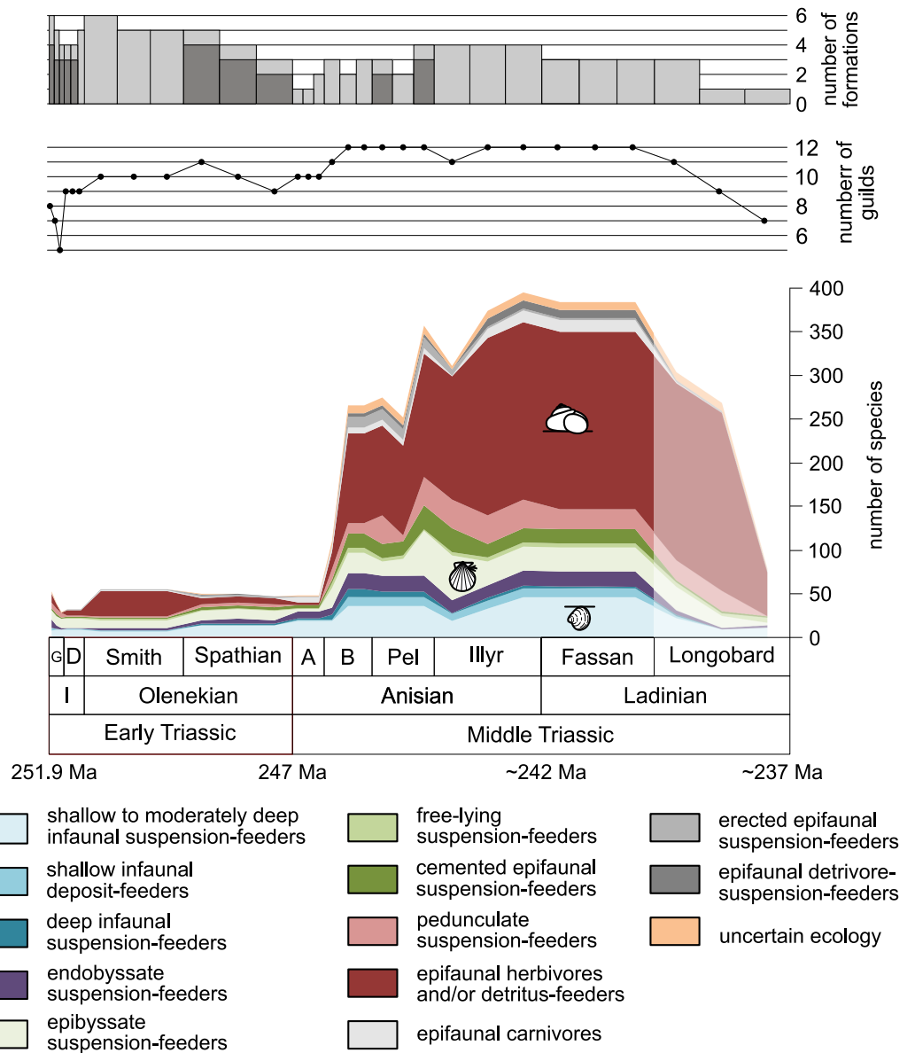
Figure 1 Maximum species richness throughout the Early and Middle Triassic. The Longobardian is palish to indicate that the decrease of species richness is not a primary signal. Light grey bars on top indicate the number of lithological units representing each time interval. In cases where information does not come from all lithological units representing the corresponding time interval, the actual number of lithological units from which information comes from is indicated by dark grey bars. Abbreviations: A, Aegean; B, Bithynian; D, Dienerian; Fassin, Fassinian; G, Griesbachian; I, Induan; Illyr, Illyrian; Longobard, Longobardian; Pel, Pelsonian; Smith, Smithian. Absolute ages according to Cohen et al., (2013, updated) and Ovtcharova et al. (2015) . Information about the relative duration of substages come from Nawrocki & Szulc (2000) , Götz, Szulc & Feist-Burkhardt (2005) , Galfetti et al. (2007) , Ovtcharova et al. (2006) and Widmann et al. (2020) . Symbols for ecological guilds redrawn after Aberhan (1994) . See text for further explanation.
