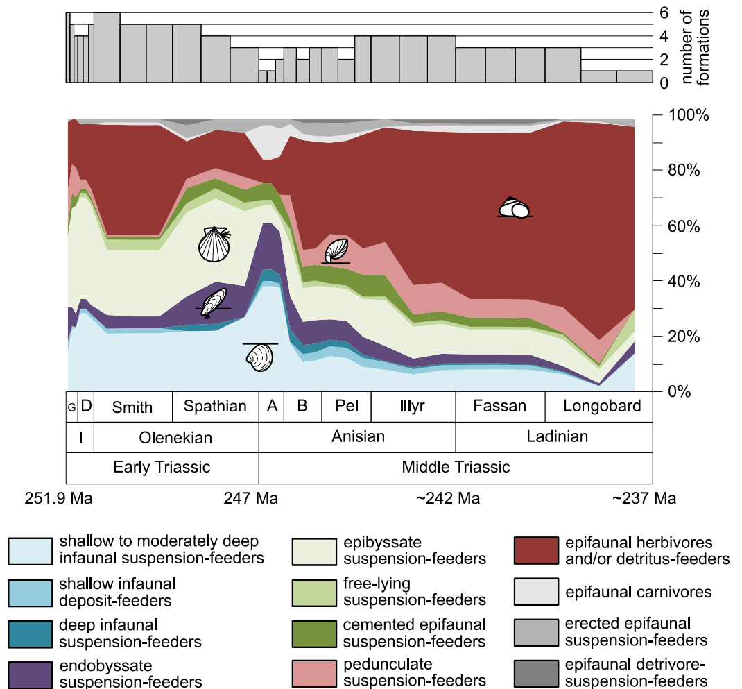
Figure 3 Guild-species diversity throughout the Early and Middle Triassic. Bars on top indicate the number of lithological units representing each time interval. Abbreviations, symbols for ecological guilds and information about the relative duration of substages as in Fig. 1. See text for further explanation.
