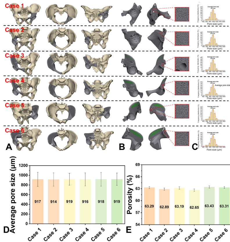
Figure 2. (A) Three-dimensional models of the reconstructed pelvis at the anteroposterior, inlet and outlet views. (B) The prosthesis models with delicate-defined solid architecture and porous structure. (C) The distribution of the pore size ranging from 500 to 1400 \mu\text{m} . (D, E) The average pore size (D) and the porosity (E).
