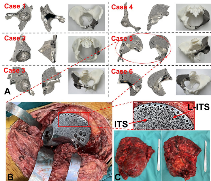
Figure 5. (A) The photographs of prostheses fabricated by EBM. (B, C) Intraoperative photographs of tumour resection and prosthesis implantation. EBM: electron beam melting; ITS: Imitation of trabecular structure; L-ITS: large pore size imitation of trabecular structure.
