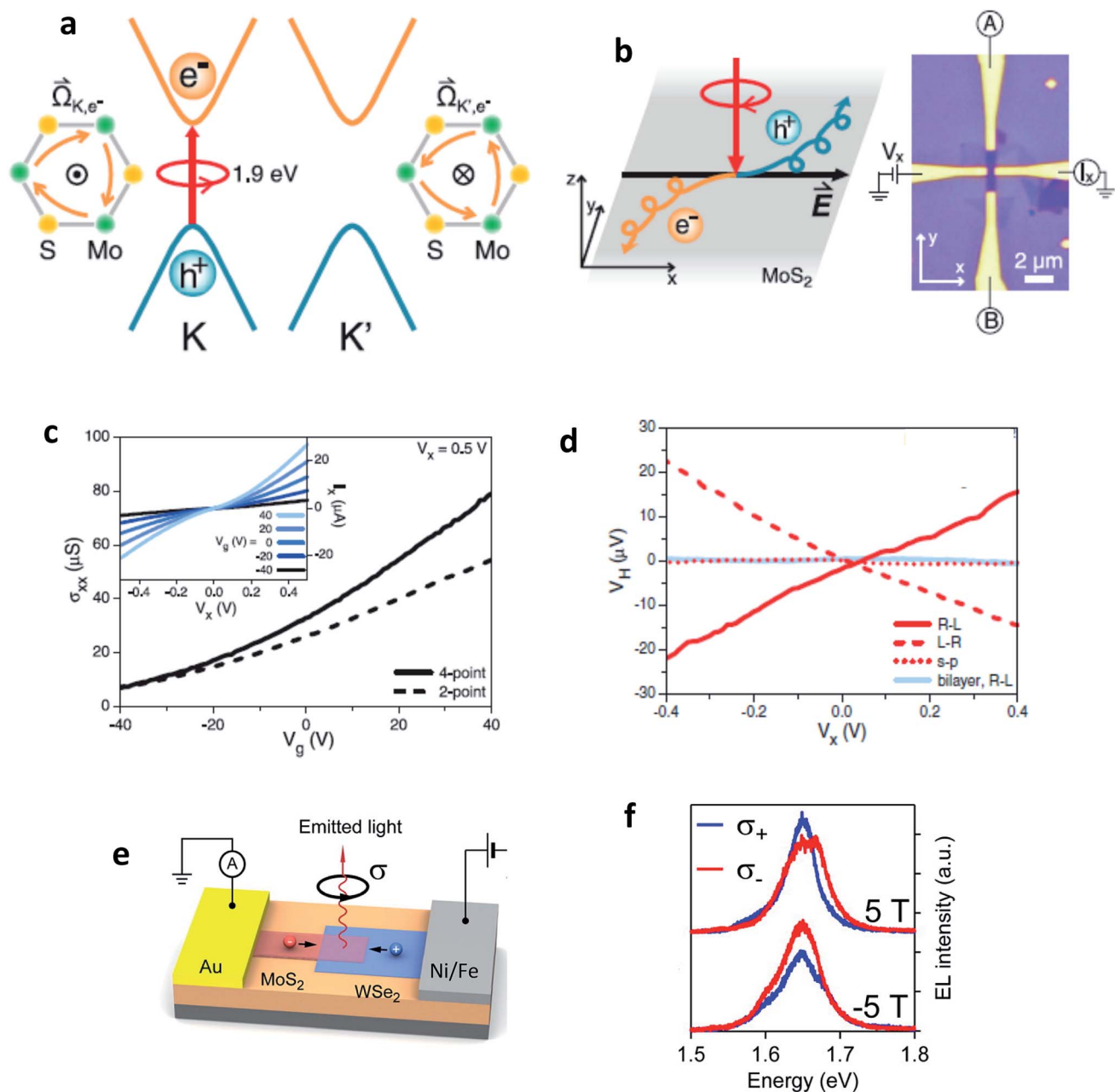
Fig. 11 Valley Hall effect based optoelectronics. (a) Schematics of valley-dependent optical selection rules and the electrons at the K and K' valleys that possess opposite Berry curvatures \vec{\Omega} . The orange arrows represent clockwise hopping motions of the K and K' electrons. (b) Experimental demonstration of photoinduced valley Hall effect with the image of a Hall bar device. (c) Two-point (dashed line, V_x = 0.5 V) and four-point (solid line) conductivities of the device as a function of back gate voltage V_g . (Inset) Source–drain bias ( V_x ) dependence of the current along the longitudinal channel ( I_x ) at different back gate voltages V_g . (d) In monolayer MoS 2 , the sign of photovoltage produced in a Hall bar depends on the helicity of light, whereas the effect is absent in a bilayer or for linear polarization (Fig. 10(a)–(d): adapted with permission from ref. 193 Copyright 2014 American Association for the Advancement of Science). (e) Valley polarization by spin injection. Monolayer WSe 2 is contacted using a ferromagnetic electrode (permalloy). MoS 2 is transferred on top of the MoS 2 channel, forming a heterojunction diode. Under the application of a positive bias voltage to the permalloy electrode, holes are injected from the permalloy electrode and recombine in the junction with electrons injected from the MoS 2 side, resulting in light emission. (f) Spin-polarized charge carrier injection from a ferromagnetic electrode into a vdW heterostructure light emitter leads to circularly polarized light emission that can be tuned by an external magnetic field. (Fig. 10(e) and (f): adapted with permission from ref. 178 Copyright 2016 ACS Publications).
