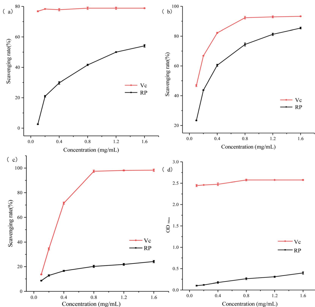
Fig. 8 Antioxidant activity of RP: (a) scavenging activity to DPPH radicals; (b) scavenging activity to ABTS radicals; (c) scavenging activity to hydroxyl radicals; (d) reducing power.
