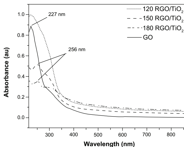
Figure 1 Ultraviolet-visible absorption spectra of reduced graphene oxide/titanium dioxide nanocomposites and graphene oxide.
