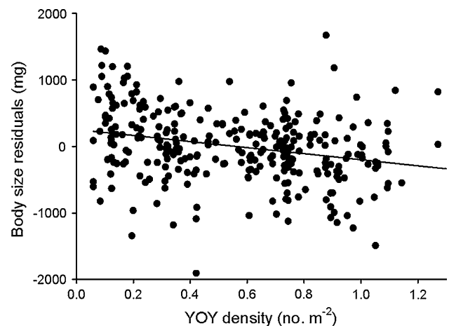
Fig. 4 Relationship between Atlantic salmon parr body growth (measured as residuals from relationship between initial and final mass) and YOY density (measured over 16 m) in Glen Meinich. Regression line is added for illustrative purpose
