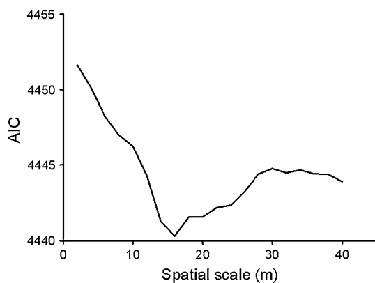
Fig. 3 AIC values of the linear mixed model describing variation in Atlantic salmon final body mass in Glen Meinich as a function of YOY densities when these were calculated over different spatial scales
