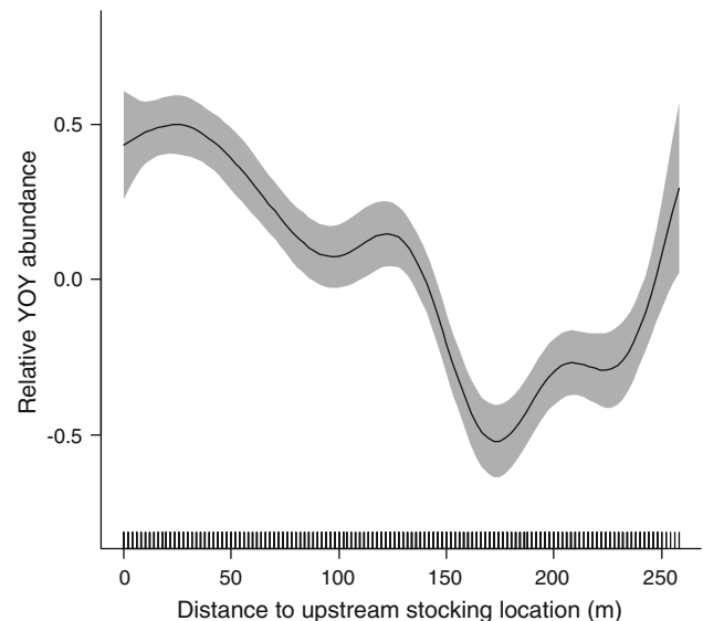
Fig. 2 Estimated smoothing curve (shaded area represents 95% confidence interval) for the best generalized additive model describing the spatial variation in YOY Atlantic salmon abundance in Glen Meinich as a function of distance to the nearest upstream stocking location while controlling for parametric terms (see Table 1). Etchings on the inside of the x-axis indicate locations of data points. Effective degrees of freedom for the smoother are 7.73, and the significance is P < 0.001
