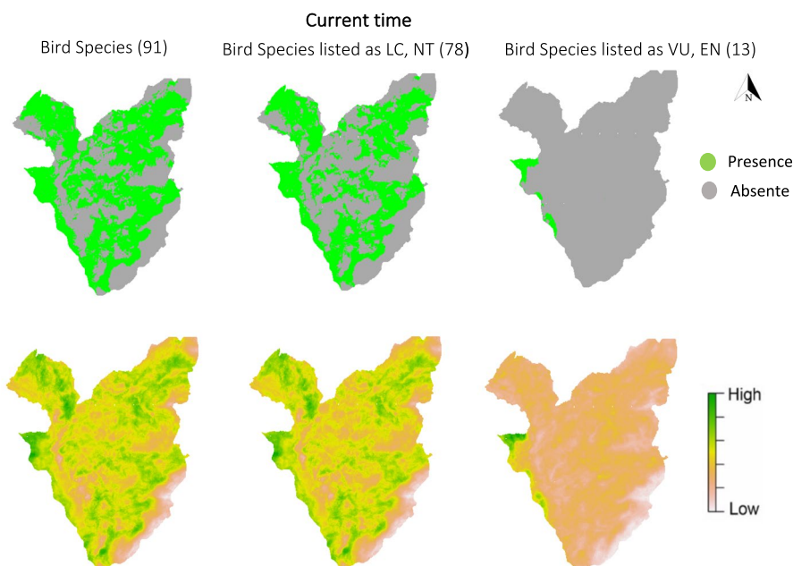
FIGURE 8 Prediction of the models for three groups of species. (i) Binary prediction of the ensemble of small models (ESMs) (upper row). (ii) The final prediction of the ESMs (lower row)
