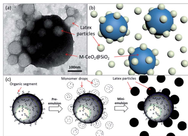
Fig. 4 (a) A TEM image of PF/ M\text{-CeO}_2@\text{SiO}_2 particles; schematic representations of (b) PF/ M\text{-CeO}_2@\text{SiO}_2 particles and (c) the growth of PFA latex particles.
