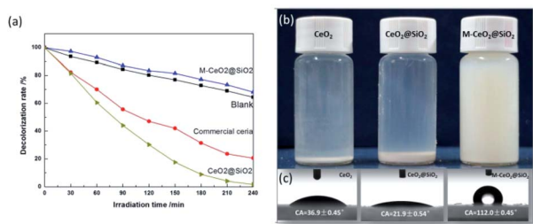
Fig. 3 Performance of the synthesized nanoparticles: (a) the photocatalytic degradation of Rh B; (b) the dispersion of \text{CeO}_2 , \text{CeO}_2@\text{SiO}_2 and M\text{-CeO}_2@\text{SiO}_2 (1 wt%) in monomer mixtures; and (c) the water contact angles of \text{CeO}_2 , \text{CeO}_2@\text{SiO}_2 and M\text{-CeO}_2@\text{SiO}_2 .
