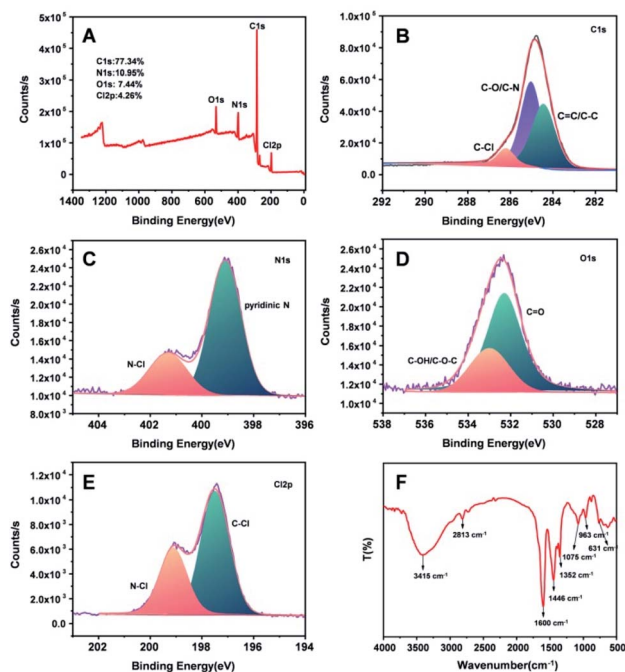
Fig. 2 XPS survey (A), XPS high-resolution surveys of C 1s (B), N 1s (C), O 1s (D) and Cl 2p (E), and FTIR spectrum (F) of CDs.
