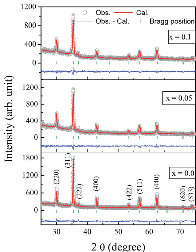
Fig. 2 Rietveld refined X-ray diffraction patterns of \text{Co}_{0.7}\text{Zn}_{0.3}\text{Gd}_x\text{-1}\text{Fe}_{2-x}\text{O}_4 ( x = 0.0, 0.05, 0.1 ). The Bragg peak positions are shown in green at the bottom of the XRD patterns. These Bragg peaks are correlated to the space group Fd\bar{3}m for \text{Co}_{0.7}\text{Zn}_{0.3}\text{Gd}_x\text{Fe}_{2-x}\text{O}_4 .
