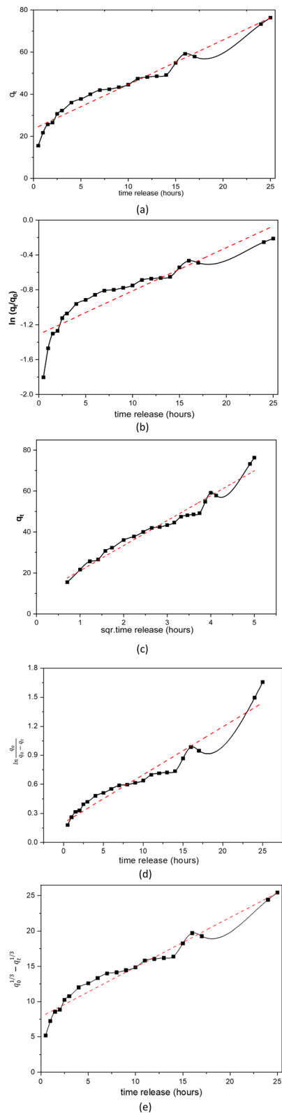
Fig. 11 Linear curves of rifampicin pH 6.5 release kinetics (a) zero order, (b) first order, (c) Higuchi model, (d) Kitazawa model, and (e) Hixon–Crowell model.
