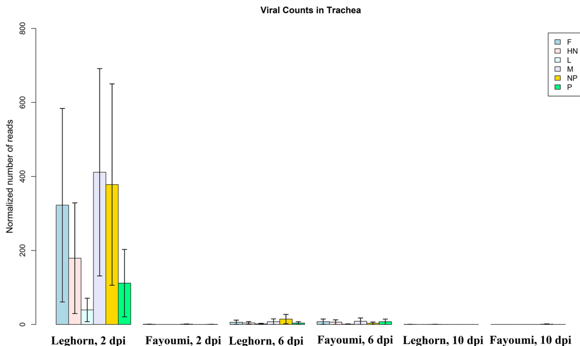
Figure 1. Normalized number of reads that aligned to specific gene segments of the La Sota Newcastle Disease viral genome found in the trachea; epithelium transcriptome: Fusion glycoprotein (F), Hemagglutinin-neuraminidase (HN), RNA-directed RNA polymerase L (L), Matrix protein (M), Nucleoprotein (NP), and Phosphoprotein (P). Reads were extracted from treated individuals by genetic line and time point and aligned to the NDV La Sota genome. Bars indicate normalized number of reads with standard error. A higher number of reads aligned to the viral genome in Leghorn at 2 dpi, while at 6 dpi both lines observed detected viral transcripts, with no reads detectable in either line at 10 dpi.
