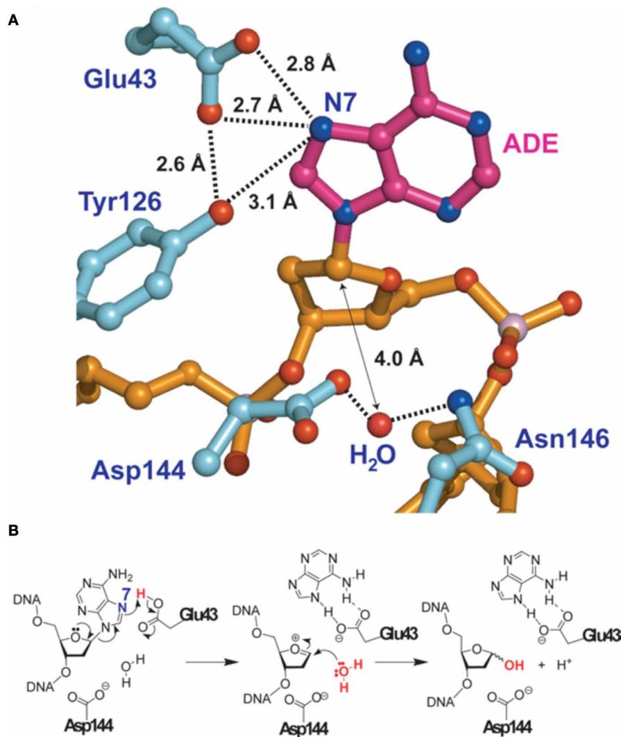
FIGURE 2 | Adenine removal by MUTYH. (A) View of the substrate adenosine interacting with catalytic residues of MUTYH. (B) Proposed glycolytic mechanism based on the structural information of (A) . Reproduced from Lee and Verdine (2009). For details see text.
