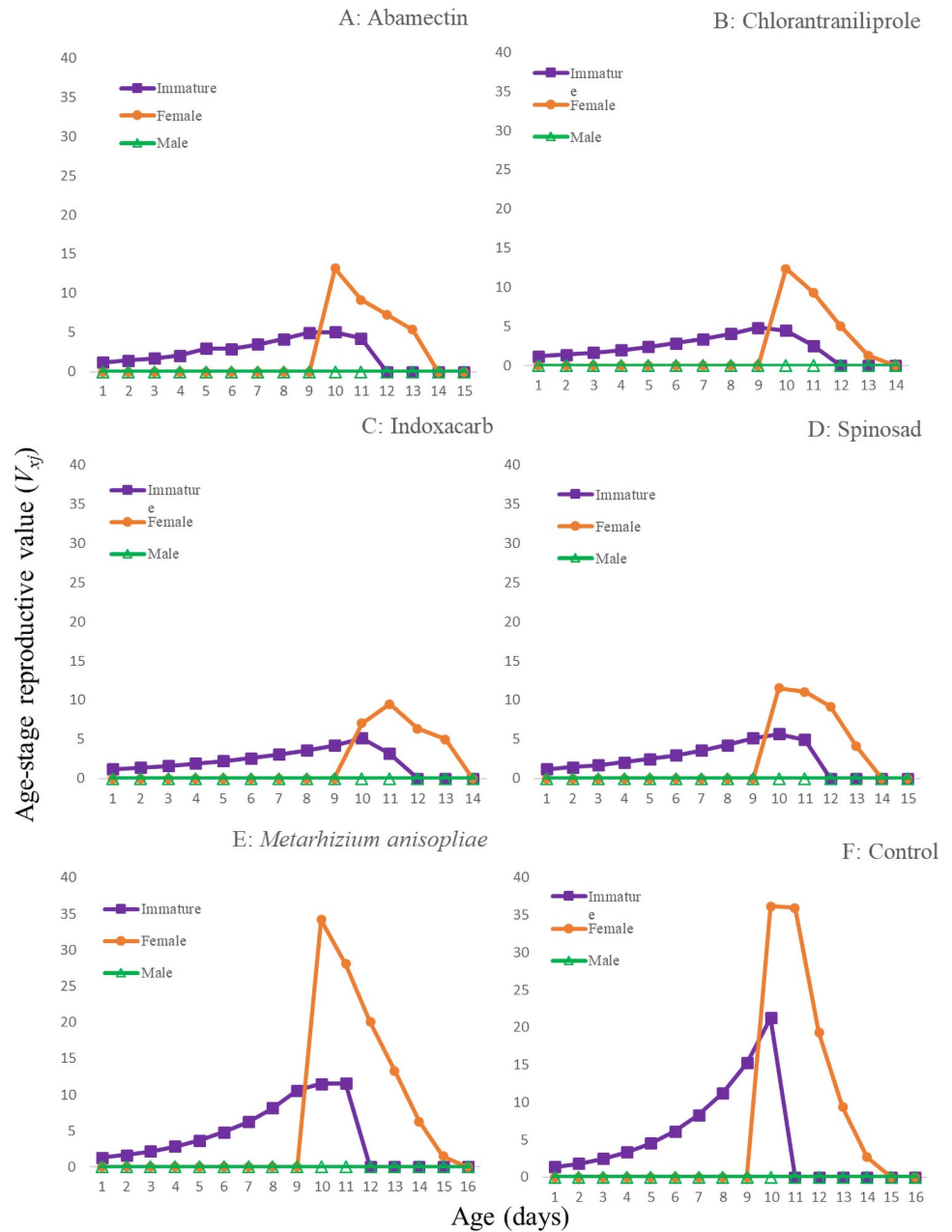
Fig 4. Age-stage reproductive value ( V_{xy} ) of the T. brassicae exposed to different pesticides 48 hours after spraying, A: Abamectin, B: Chlorantraniliprole, C: Indoxacarb, D: Spinosad, E: M. anisopliae , F: control.
