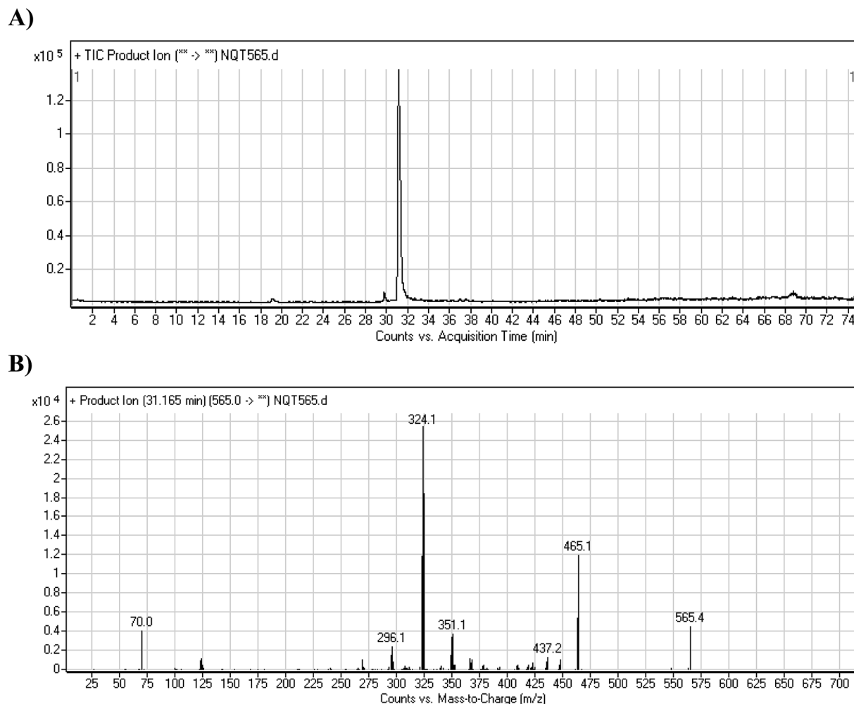
Fig. 4 PI chromatogram of the NQT565 peak at 31.2 min (A). PI mass spectrum of NQT565 (B).
