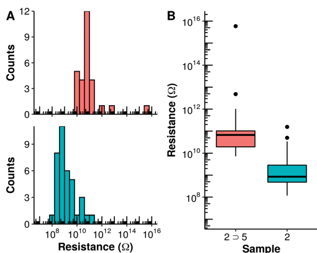
Fig. 4 Histograms (A) and boxplots (B) of the vertical resistance of monolayers of 2 (cyan) and 2 ⊃ 5 (salmon) obtained from the slope of the I–V curves measured using C-AFM at low bias and an applied force of 18 nN. In (B), the median resistance is represented by the solid lines. Black dots represent experimental points which are at a distance higher than 1.5 times the interquartile range from the hinge.
