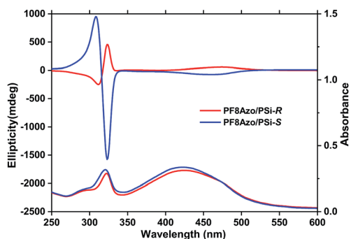
Fig. 2 The CD and UV-vis spectra of PF8Azo/PSi- S (blue line) or PF8Azo/PSi- R (red line) hetero-aggregates. The hetero-aggregates were present at 1-to-1 molar ratio as repeating units in \text{CHCl}_3\text{-MeOH} (2.0/1.0, (v/v)) cosolvent. The final concentrations of [PSi- S / R ] _0 and [PF8Azo] _0 were 1.0 \times 10^{-5} M and 1.0 \times 10^{-5} M, respectively. The single sign of the broad CD bands in the visible region was assigned to the \pi\text{-}\pi^* transitions of the PF8Azo main chain induced by the chirality/helicity of the rigid rod-like helical PSI- S and PSI- R .
