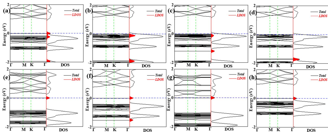
Fig. 5 The BSs and DOSs of the most stable structure of each VOC molecule on the C_6N_7 : (a) toluene-1, (b) benzene-1, (c) vinyl chloride-1, (d) ethane-1, (e) acetone-1, (f) ethanol-1, (g) acetaldehyde-1, and (h) methanal-1. The local DOS (LDOS) of isolated molecules were marked as red under total DOS curves (dark lines).
