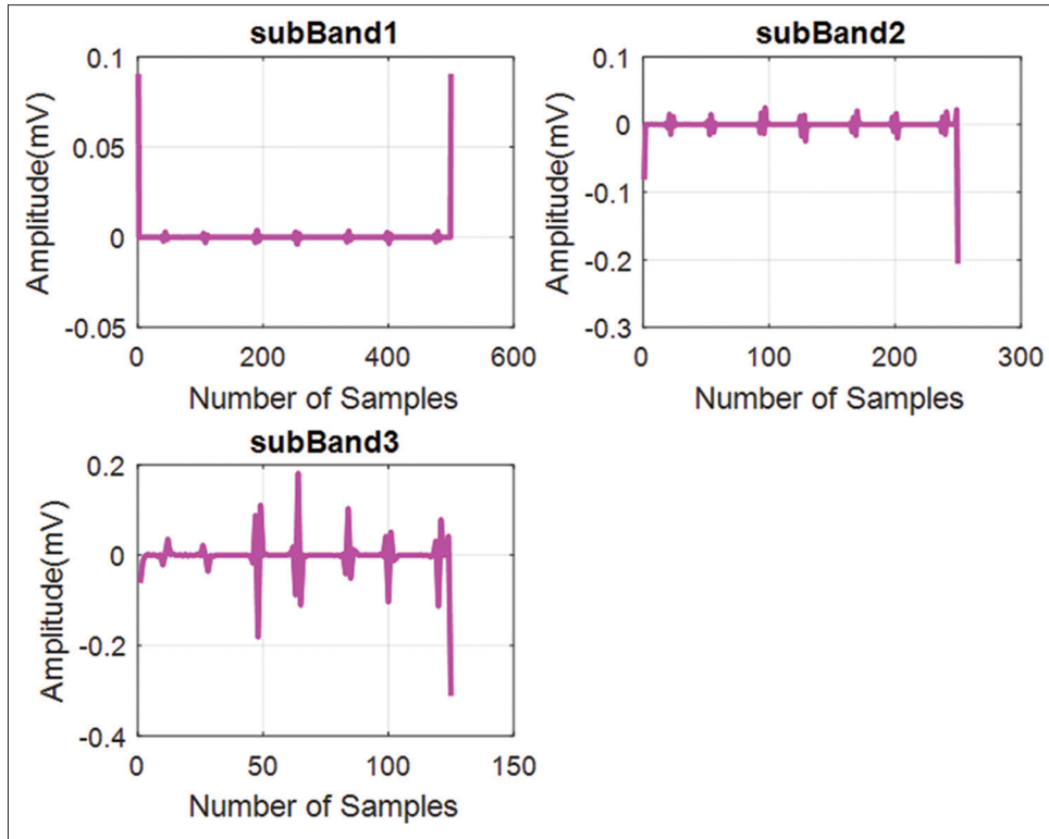
Figure 5: The sub bands of the electrocardiogram signal for Tree B
