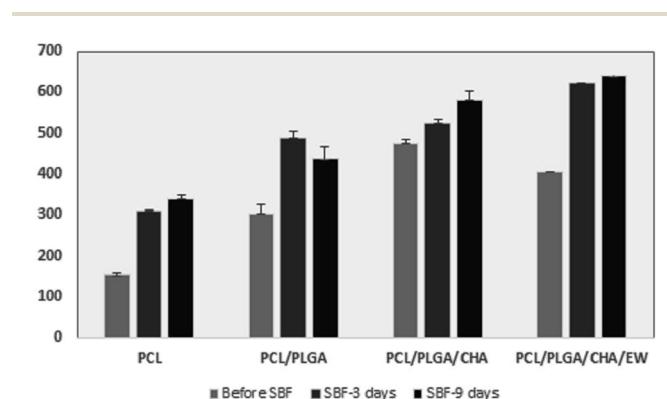
Fig. 11 Diameters of the nanofiber after immersion in the SBF for 3 and 9 days.
