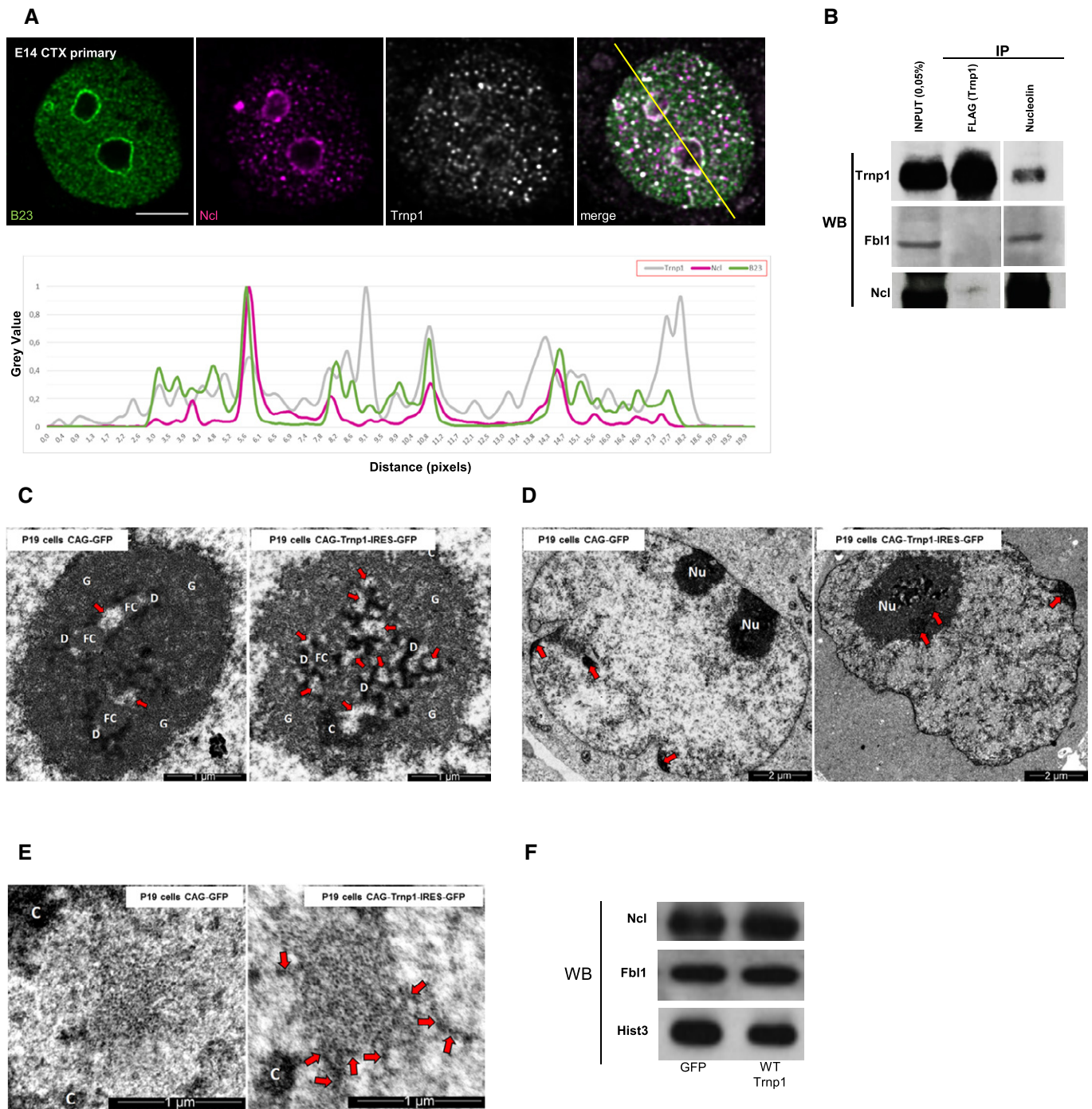
Figure 5. Trnp1 changes the architecture of nucleolus, condensed chromatin, and nuclear speckles.
