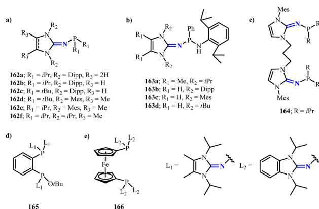
Scheme 64 Phosphine carbene complexes bearing N-heterocyclic imine group 162 – 166 .
