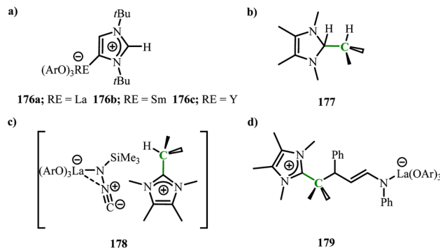
Scheme 68 Unusually NHC-stabilized rare earth aryloxide complexes 176a–176c , NHO with activated hydrogen 177 , isocyanide trimethylsilyl lanthanum amine complexes 178 and \text{La}/\text{C} 1,4-addition products 179 .
