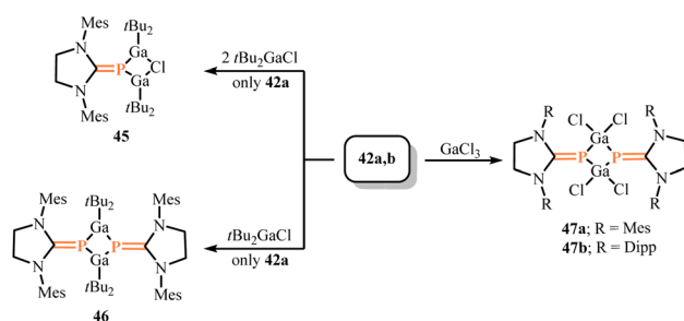
Scheme 19 Synthesis of NHCP-stabilized gallium complexes 45–47 .
