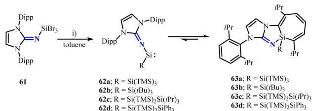
Scheme 25 Synthesis of silylenes 62 /silepins 63 . (i) For 62a : \text{KSiTMS}_3 ; for 62b : [\text{Na}\cdot(\text{THF})_2]\text{Si}t\text{Bu}_3 ; for 62c : \text{KSiTMS}_2\text{Si}(\text{iPr})_3 ; for 62d : \text{KSiTMS}_2\text{SiPh}_3 .
