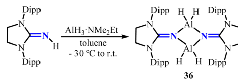
Scheme 14 Synthesis of NHI-stabilized dimeric aluminum hydride { \mu -AlH 2 } 2 ( 36 ).
