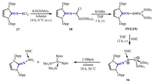
Scheme 9 Synthesis of borasilene 20 and its reaction with HBpin. NHC = 1,3,4,5-tetramethylimidazol-2-ylidene.
