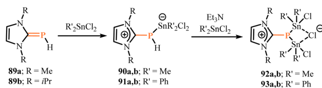
Scheme 36 Reaction of NHCP 89 with diorganotin dichlorides.
