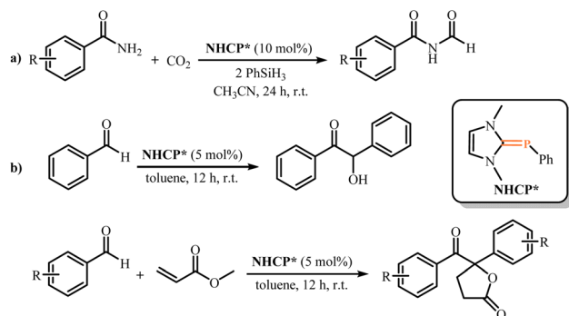
Scheme 104 (a) \text{CO}_2 activation achieved by NHCP; (b) activation of aldehydes and methyl acrylates to synthesize \gamma -butyrolactone catalyzed by NHCP.
