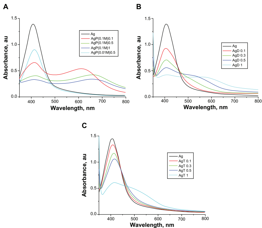
Figure 5 Optical absorption spectra of silver nanoparticles with 10^{-2} M and 10^{-1} M procaine, P (A), 10^{-2} M dibucaine, D (B), and 10^{-2} M tetracaine, T (C) solutions; volumes (mL) of anesthetic solutions added to 2 ml silver nanoparticles solution are indicated in the inserted frame.
