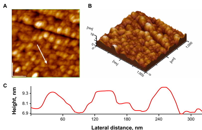
Figure 7 Atomic force microscopy images silver nanoparticles on glass in presence of 10^{-2} M dibucaine solution; scanned area 1 \mu\text{m} \times 1 \mu\text{m} : (A) 2-D topography; (B) 3-D topography; (C) profile of the cross-section along the arrow in panel A.
