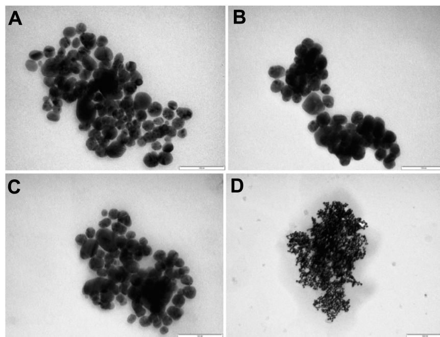
Figure 6 Transmission electron microscopy images of the silver nanoparticles with 10^{-2} M procaine (A), 10^{-3} M dibucaine (B), and 10^{-2} M tetracaine (C, D) solutions in the 1:1 volume ratio, bars in the images correspond to 100 nm (A–C), respectively to 200 nm (D).
