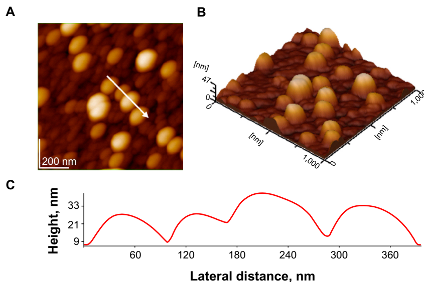
Figure 4 Atomic force microscopy images silver nanoparticles on glass; scanned area 1 \mu\text{m} \times 1 \mu\text{m} : (A) 2-D topography; (B) 3-D topography; (C) profile of the cross-section along the arrow in panel A.
