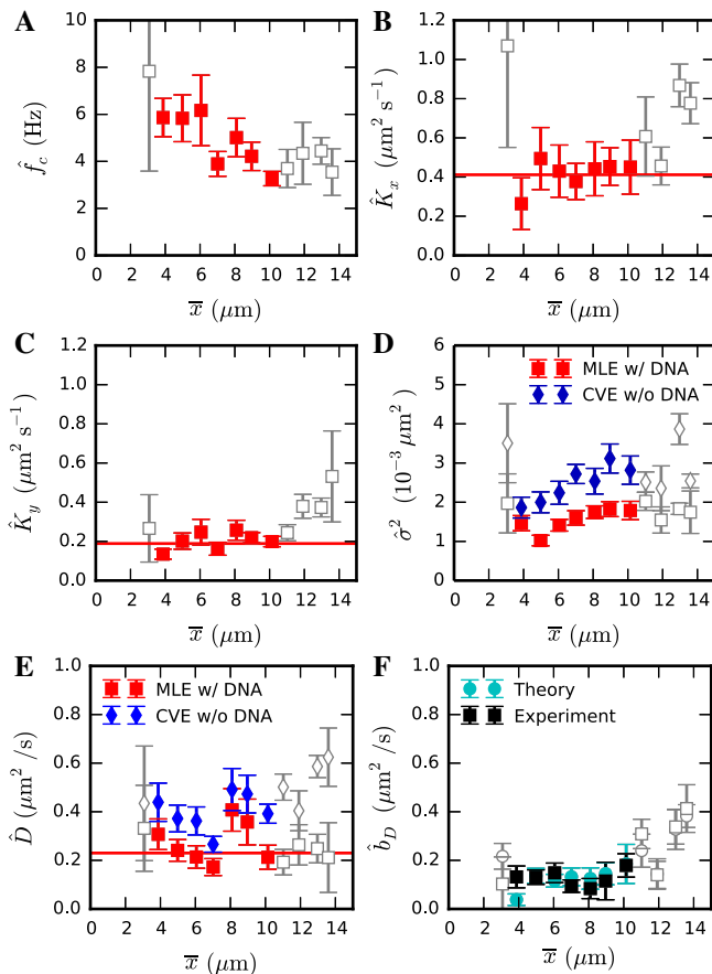
Figure 2. Estimated parameter values as functions of the protein's position \bar{x} on DNA. Results for molecule no. 5 (pH 7.5 and [\text{NaCl}] = 0.01 \text{ M} ). Averages are weighted means and error bars are weighted s.e.m., except for estimates of diffusion coefficients; their averages are simple mean values. Data close to the DNA ends (open gray symbols) are excluded in the following analysis to avoid bias (see discussion in Supplementary Section S3A). (A) MLE of the corner frequency f_c of transverse ( y -direction) DNA motion. Measured values vary by a factor two between the tethered and the free end. (The hypothesis that f_c is constant is refuted with P = 6 \times 10^{-7} .) The faster dynamics near the tethered end is due to larger tension in the DNA there. (The corner frequency of the DNA's longitudinal motion is twice the corner frequency of its transverse motion.) (B) The diffusivity K_x(\bar{s}) of longitudinal DNA fluctuations is constant along the DNA, corresponding to increasing amplitude in the downstream direction in consequence of decreasing tension; \bar{K}_x = 0.41 \pm 0.03 \mu\text{m}^2/\text{s} ( P = 0.93 ). (C) The diffusivity K_y(\bar{s}) of transverse DNA fluctuations is also constant along the DNA; \bar{K}_y = 0.19 \pm 0.02 \mu\text{m}^2/\text{s} ( P = 0.19 ). (D) The CVE overestimates \sigma^2 , the variance of localization errors, by almost a factor two because it does not account for DNA motion. The MLE of \sigma^2 increases slightly towards the free end. The assumption that it is constant has negligible support: P = 0.003 . (E) Estimated diffusion coefficients. The uncorrected CVE overestimates diffusion coefficients significantly, because it does not account for DNA motion. The MLE does not, and shows that diffusion coefficients do not depend on the protein's position on the DNA ( P = 0.10 ). (F) Experimental estimates of the bias b_D of the CVE, calculated as \hat{D}_{\text{cve}} - \hat{D}_{\text{mle}} , and theoretical estimates, calculated from Equation (1) using weighted means of estimates of f_c and K_x (Materials and Methods and Supplementary Section S3D). The theory generally agrees excellently with experiments. The bias increases near the DNA's free end, where DNA fluctuations are larger and slower.
