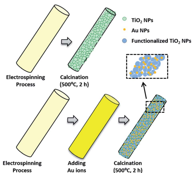
Fig. 1 Schematic diagram illustrating the formation of \text{TiO}_2 -Au composite NFs.
